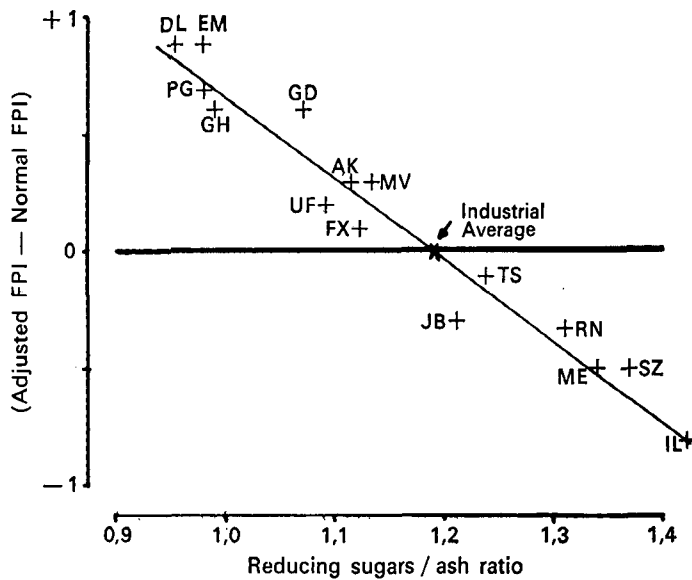
FIGURE 5 Industry 1975/76: Change from normal to adjusted Factory Performance Index versus reducing sugars/ash ratio in molasses.
