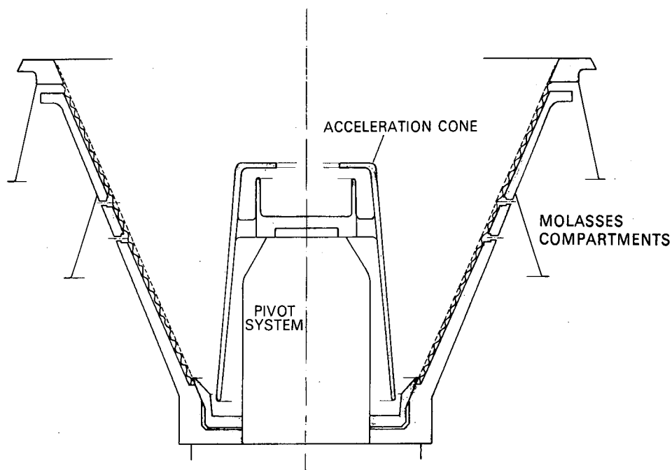
FIGURE 2 The FC 1000 GCVSE 25° basket arrangement.
