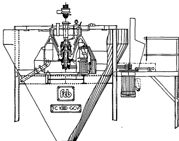
FIGURE 1 Basic features of the machine.
