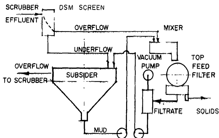
FIGURE 4 Subsider and filter.
