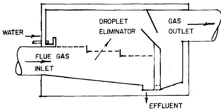
FIGURE 2 Perforated plate scrubber in brick housing.
