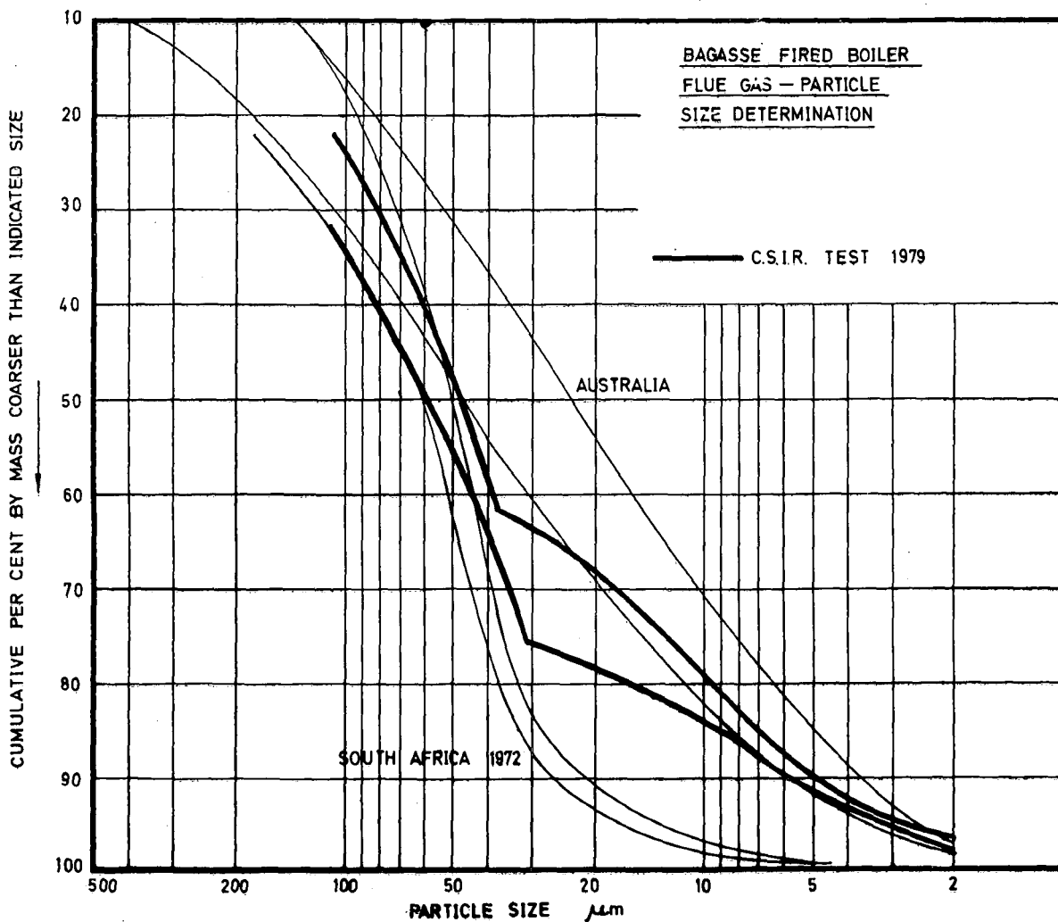
FIGURE 5 CSIR Flue Gas particle size determination.
