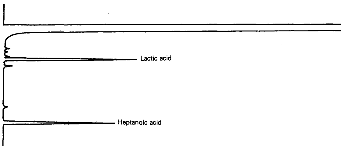
FIGURE 1 Chromatogram of lactic acid and heptanoic acid.
