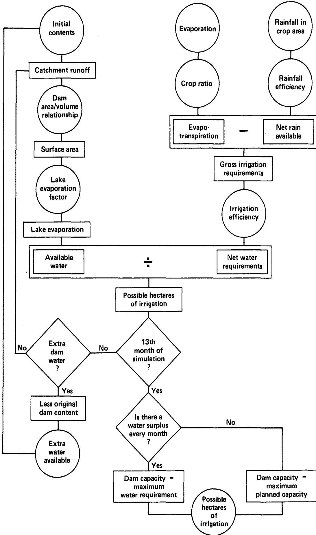
FIGURE 2 Flow chart of "Dam Full" programme.
