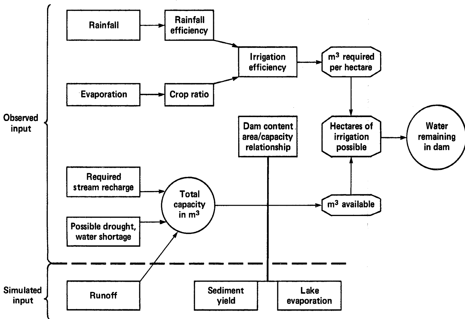
FIGURE 1 The different elements considered in the "Dam Full" model.
