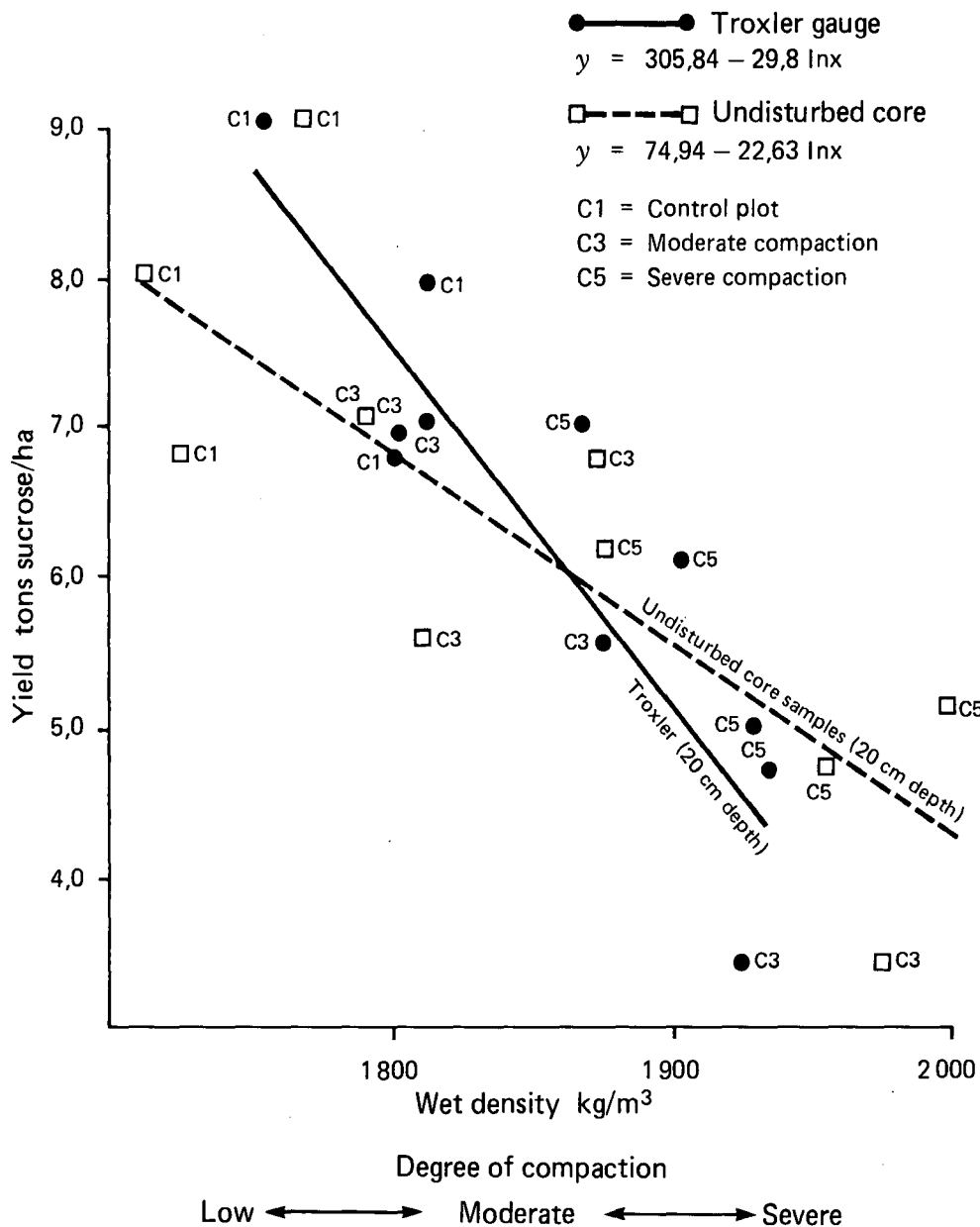
FIGURE 6 Yield in relation to soil wet density as determined by two methods.
