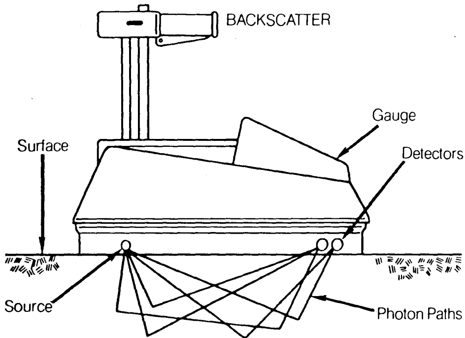
FIGURE 2 Troxler density gauge shown measuring in the backscatter mode.
