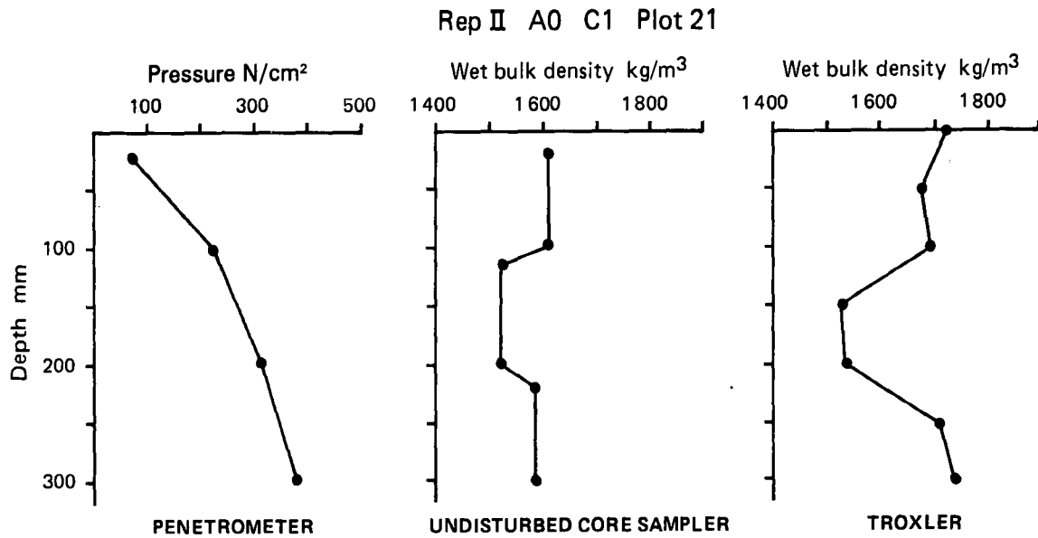
FIGURE 4 Comparison of three methods of measuring natural compactive effects to depth (Control - uncompacted treatment).
