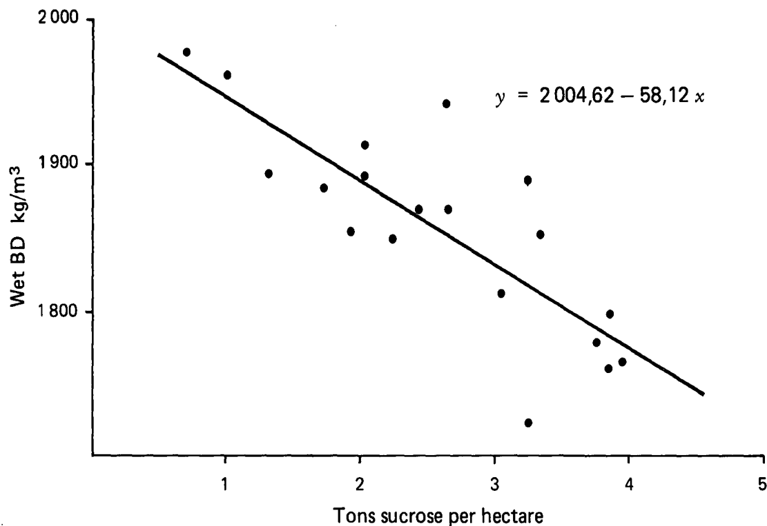
FIGURE 8 Yield in relation to Troxler wet density values at 200 mm depth (1983 crop).
