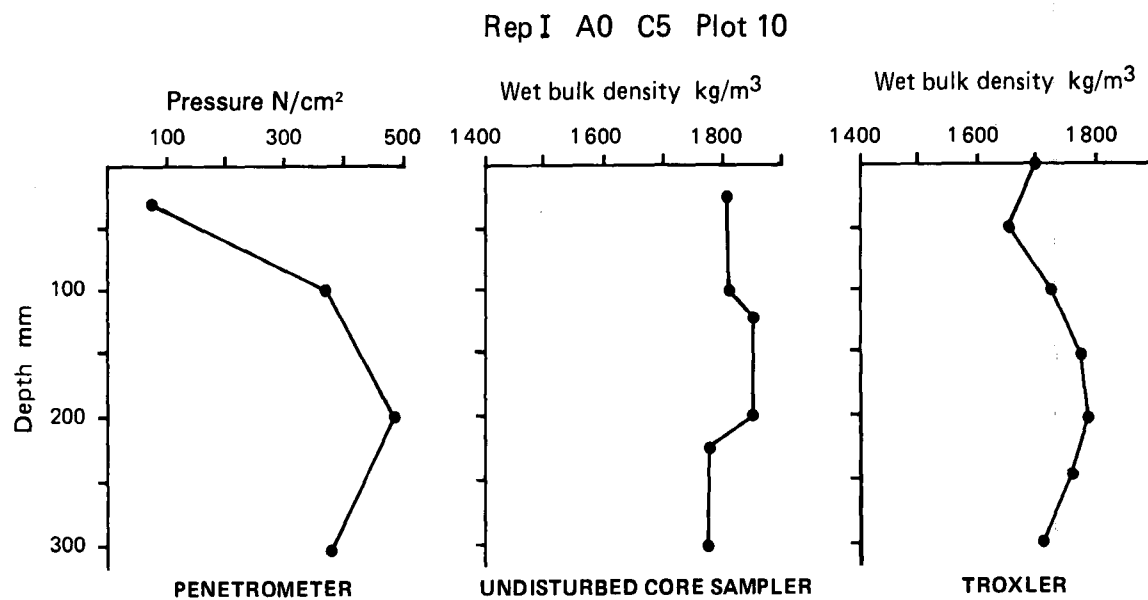
FIGURE 5 Comparison of three methods of measuring the effects of severe compaction to depth.
