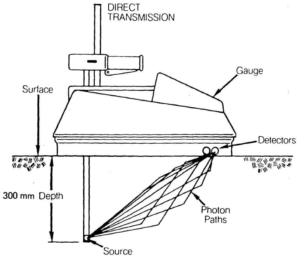
FIGURE 3 Troxler density gauge shown measuring in the direct transmission mode.
