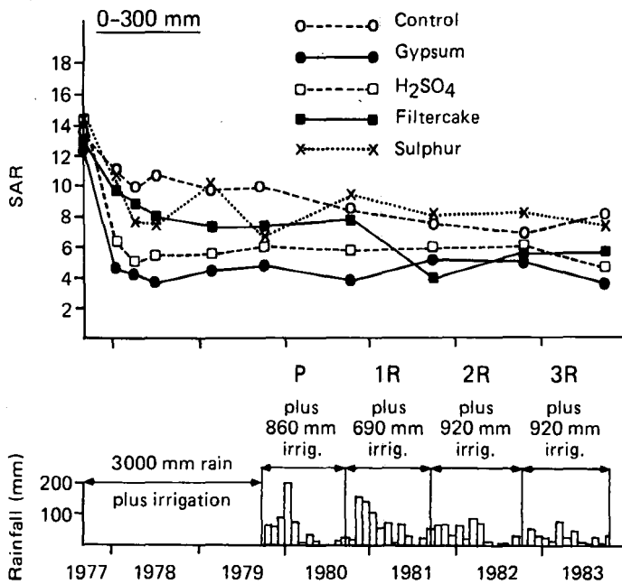
FIGURE 1 Changes in topsoil SAR values with time.
