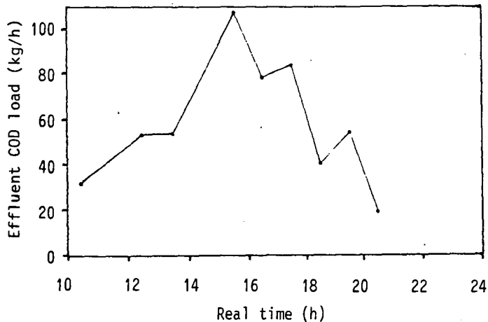
FIGURE 4 Chemical oxygen demand of the final effluent during the test
