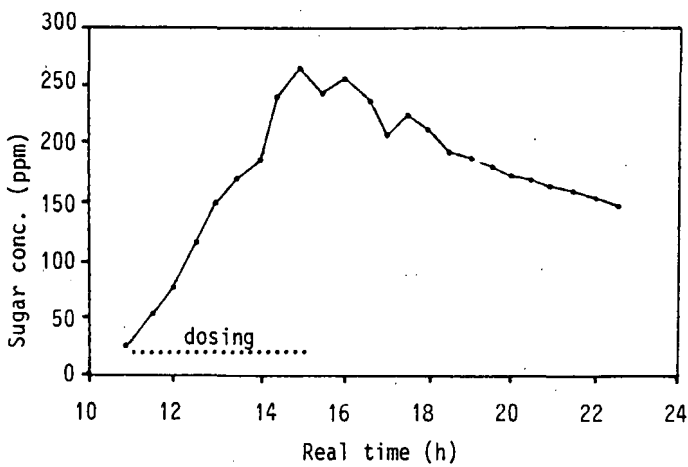
FIGURE 2 Sugar concentrations in condenser water during and after dosing
