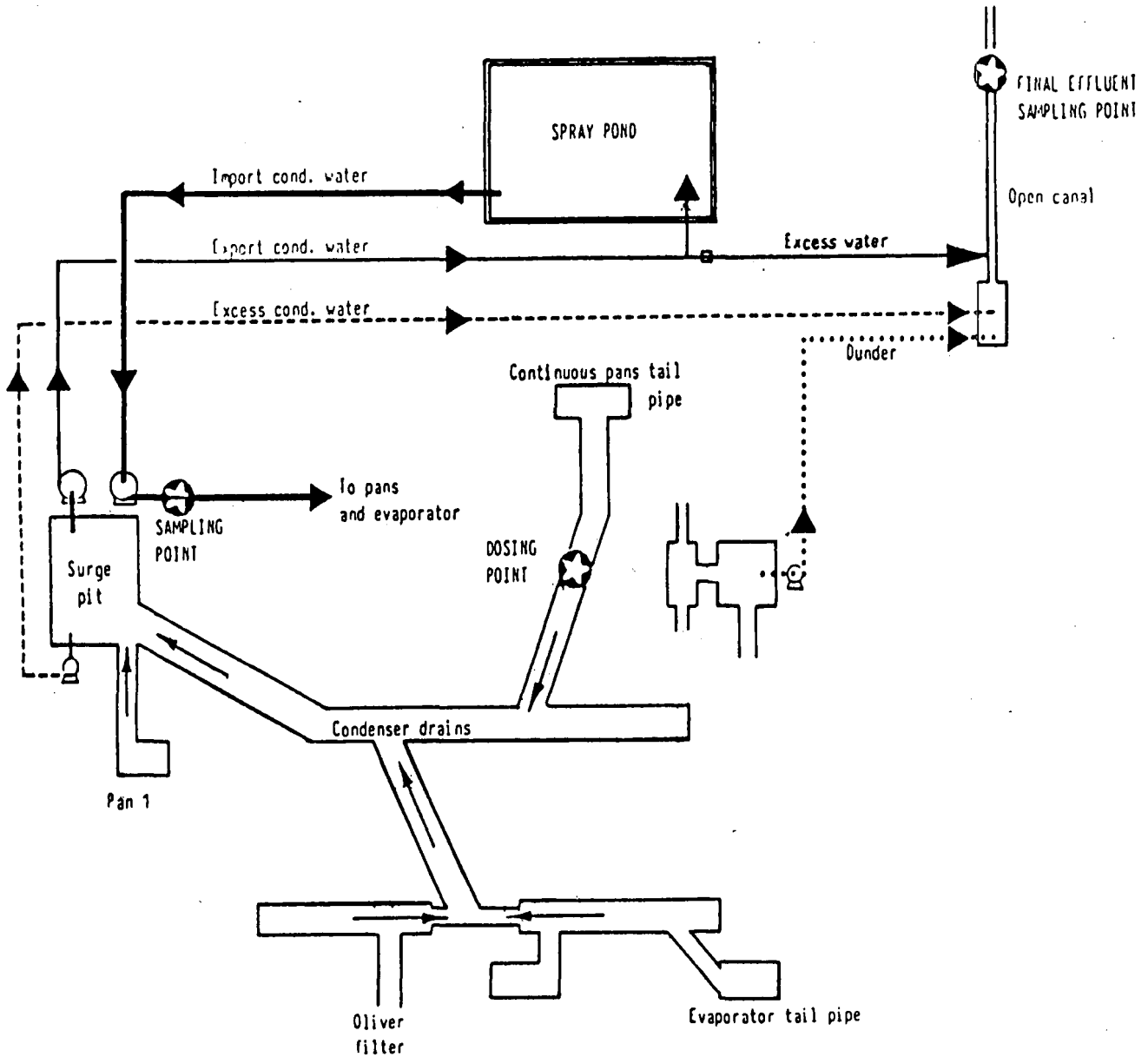
FIGURE 1 Simplified diagram of the condenser water circuit showing dosing and sampling points
