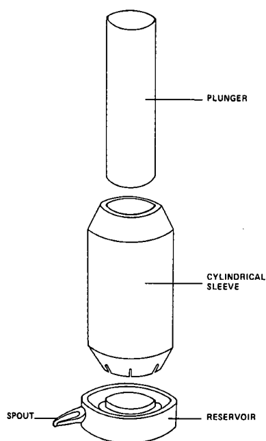
FIGURE 4 Isometric drawing of plunger, sleeve and reservoir
