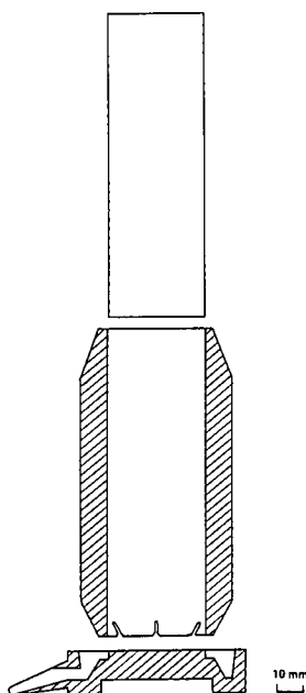
FIGURE 3 Cross-section of the stainless steel tool used in the hydraulic leaf press
