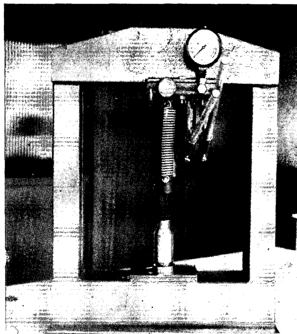
FIGURE 1 Hydraulic ram press for extracting fluids from leaf tissue
