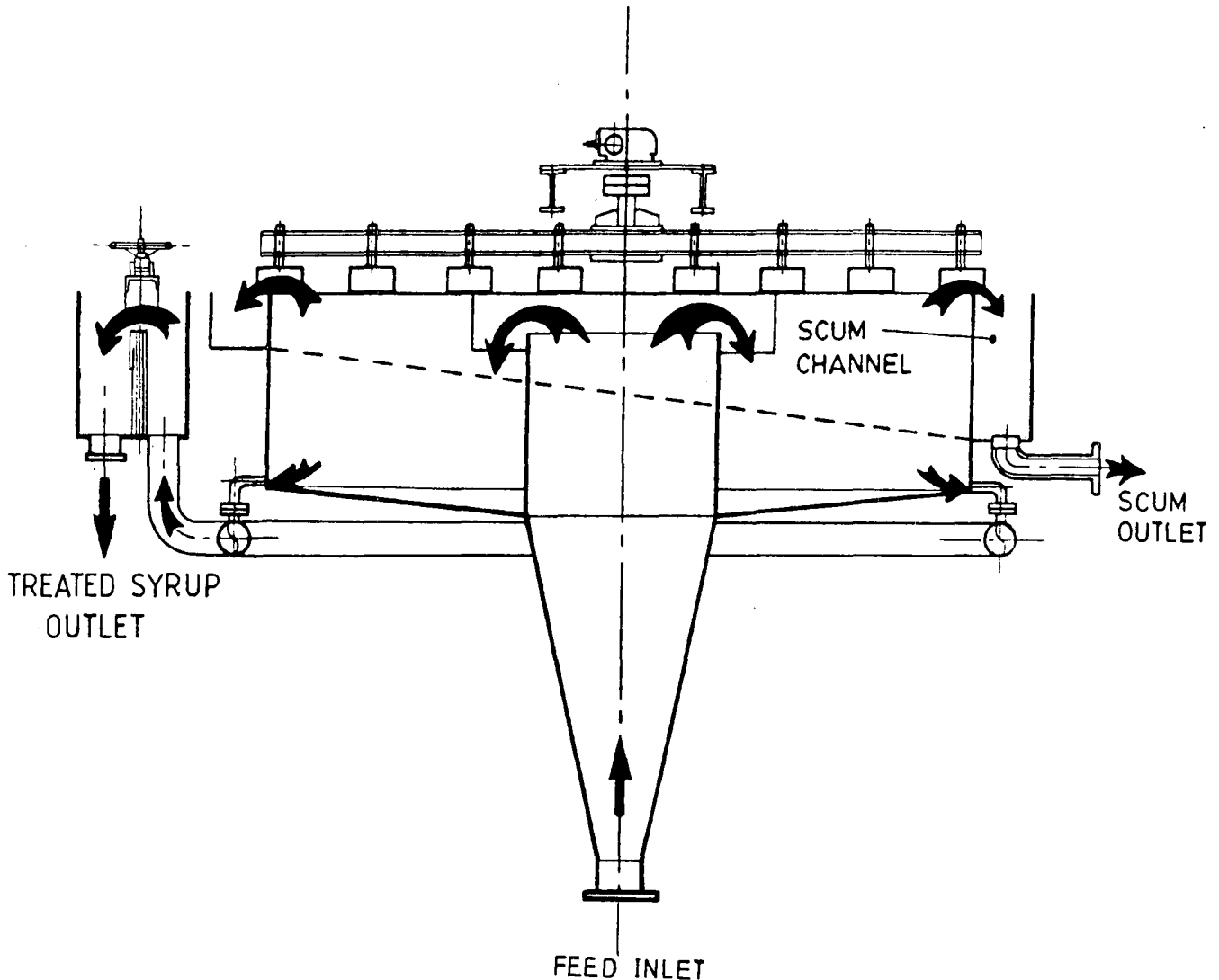
FIGURE 4 Sketch of the syrup clarifier installed at Empangeni.
