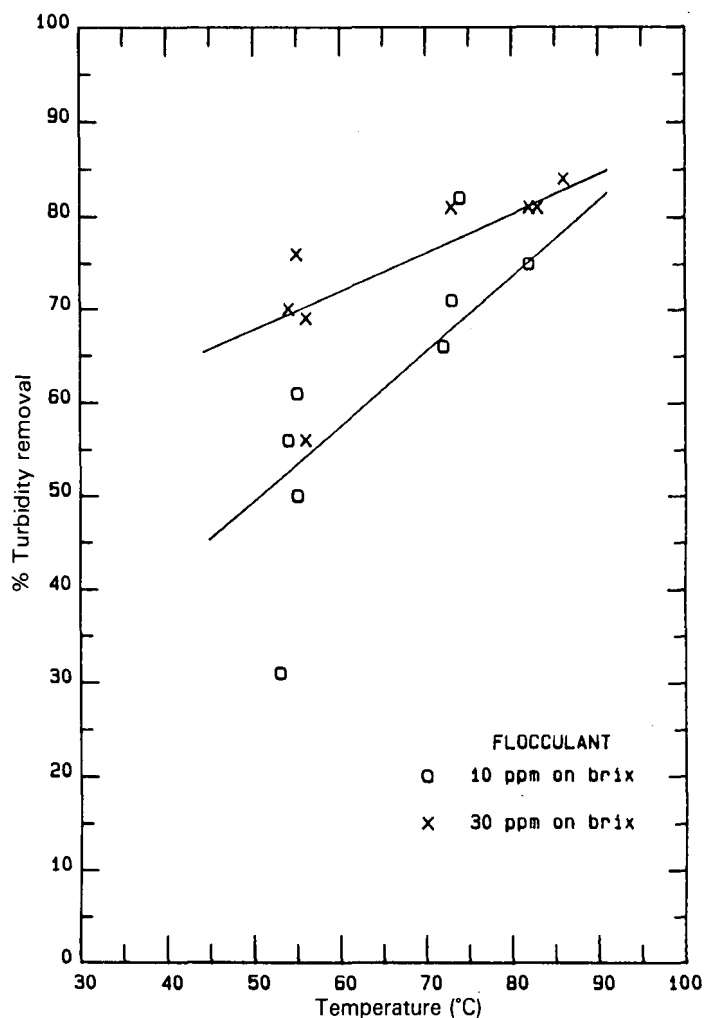
FIGURE 10 Effect of temperature and flocculant dosing level on performance of the Empangeni syrup clarifier.
