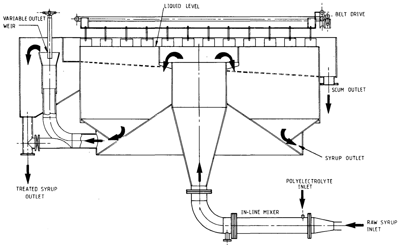
FIGURE 13 Sketch of the syrup clarifier installed at Triangle, Zimbabwe.
