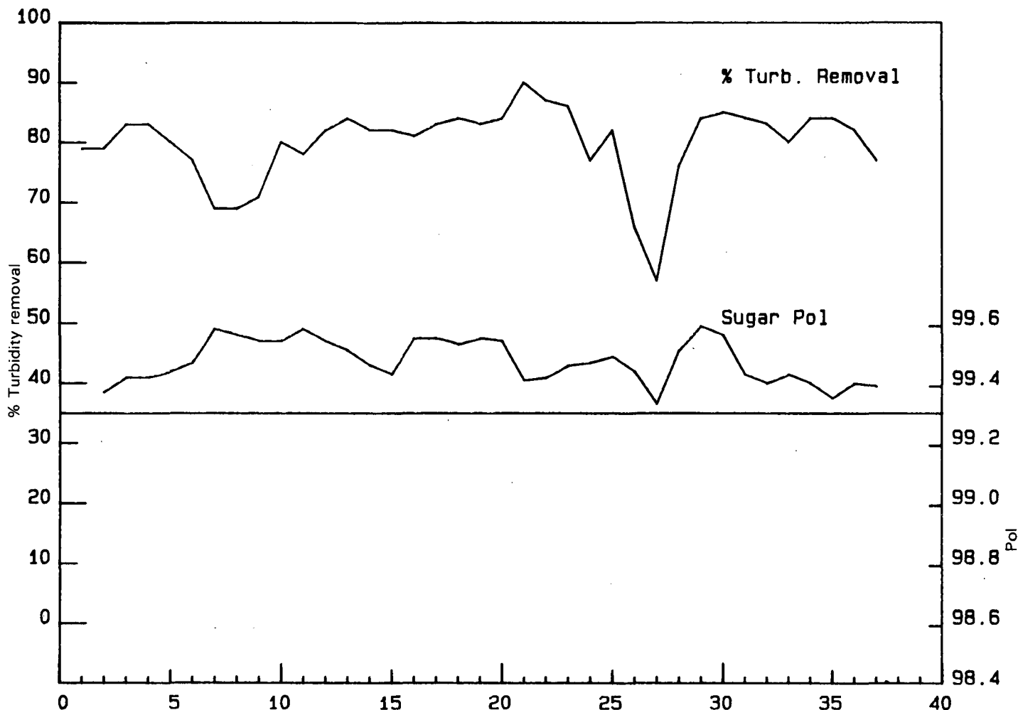
FIGURE 7 Operational results at Empangeni, 1982/83 season.
