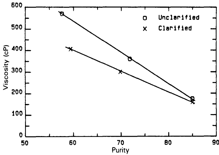
FIGURE 3 Viscosity of syrup and molasses (at 73 brix and 40 °C) with and without syrup clarification.
