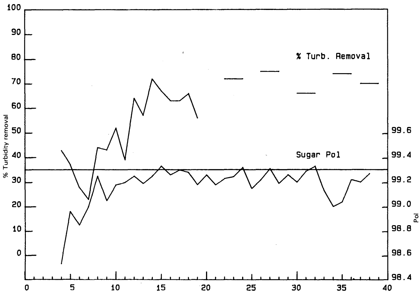
FIGURE 6 Operational results at Empangeni, 1981/82 season.
