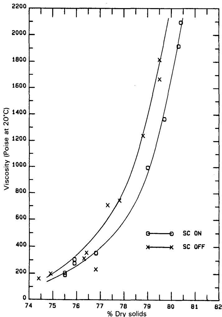
FIGURE 9 Final molasses viscosities measured at Empangeni during the 1981/82 season.
