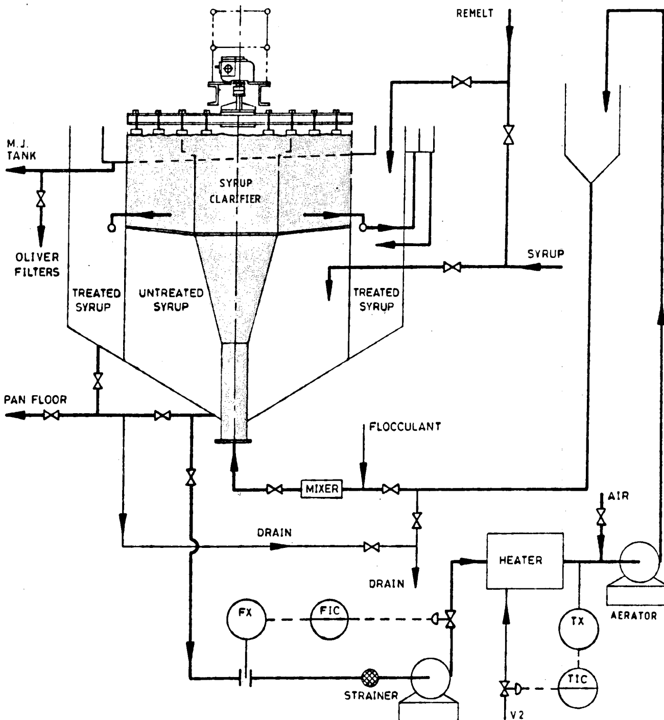
FIGURE 5 Flow diagram for Empangeni syrup clarification.
