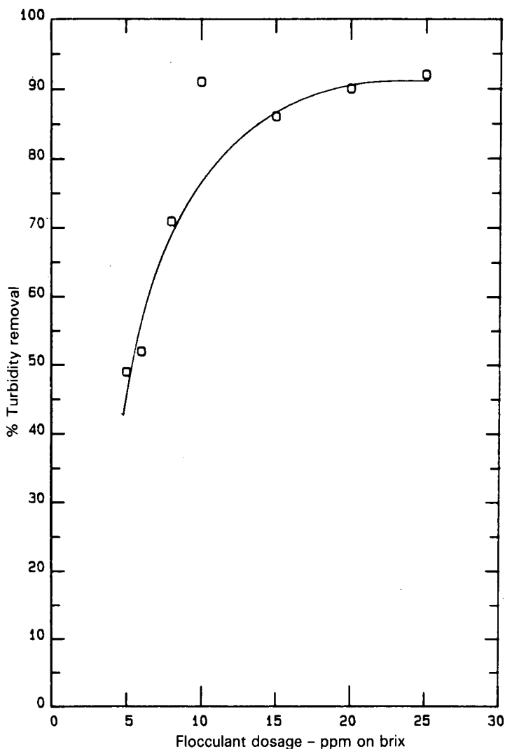
FIGURE 1 Turbidity removal measured in the laboratory as a function of flocculant dosage.
