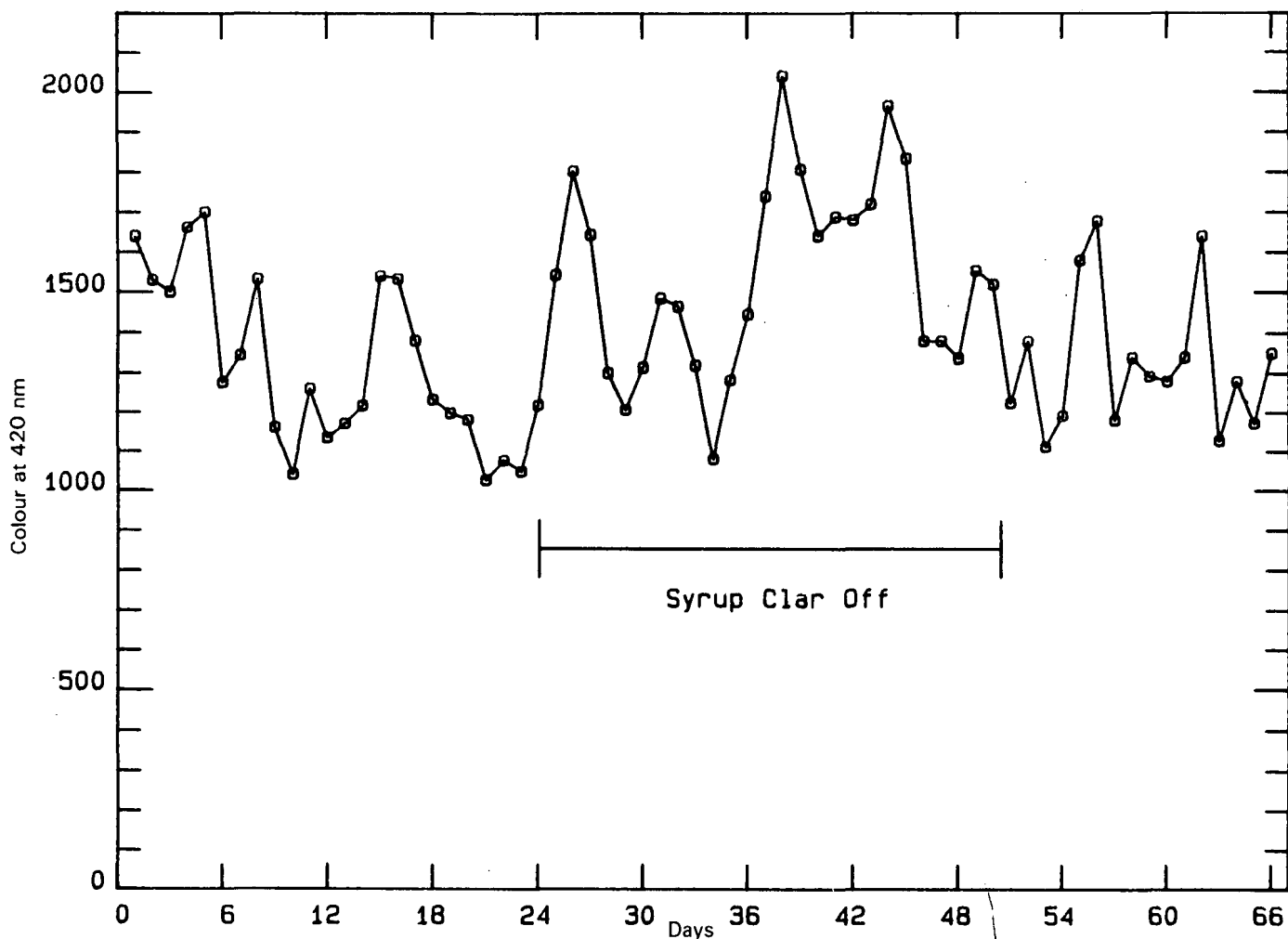
FIGURE 12 Colour of Felixton sugar delivered to the Refinery including a period when the syrup clarifier was taken off.
