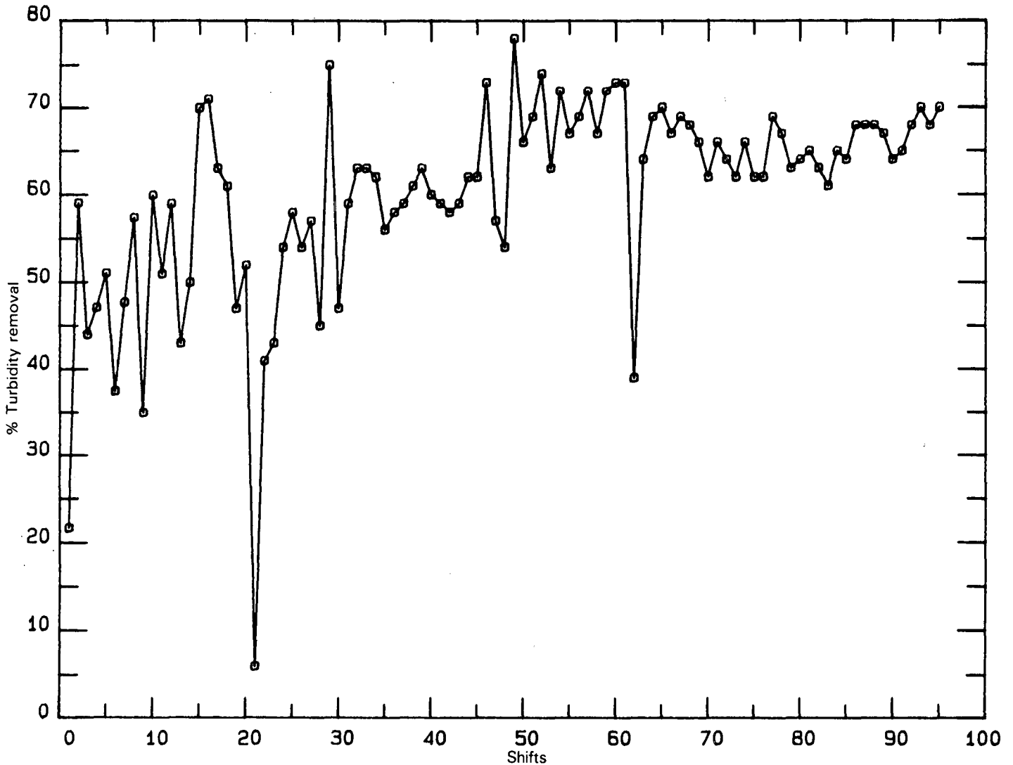
FIGURE 11 Turbidity removal measured in the Felixton syrup clarifier, average temperature 58 °C, during a test period.
