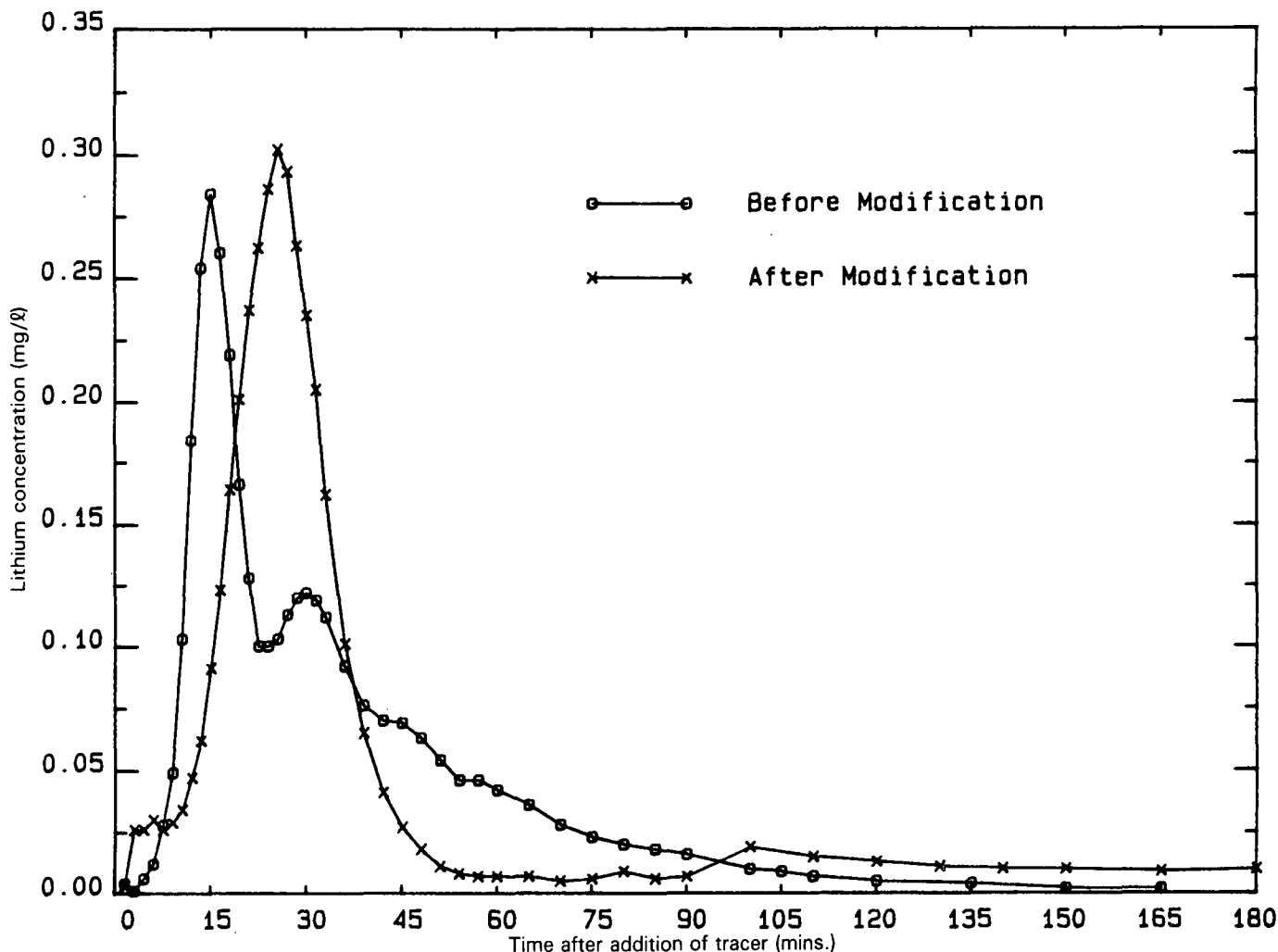
FIGURE 8 Residence time distribution of syrup measured in the Empangeni syrup clarifier before and after modification to the offtakes.
