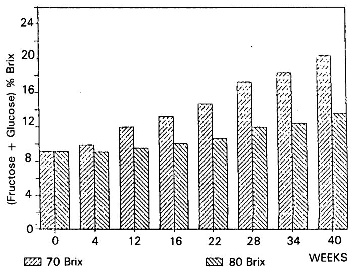
FIGURE 4 Invert formation: B molasses at 45°C
