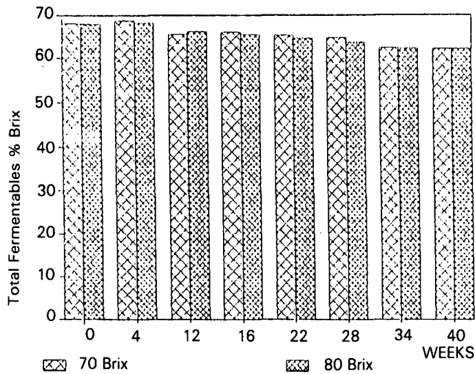
FIGURE 5 Total fermentables: B molasses at 45°C
