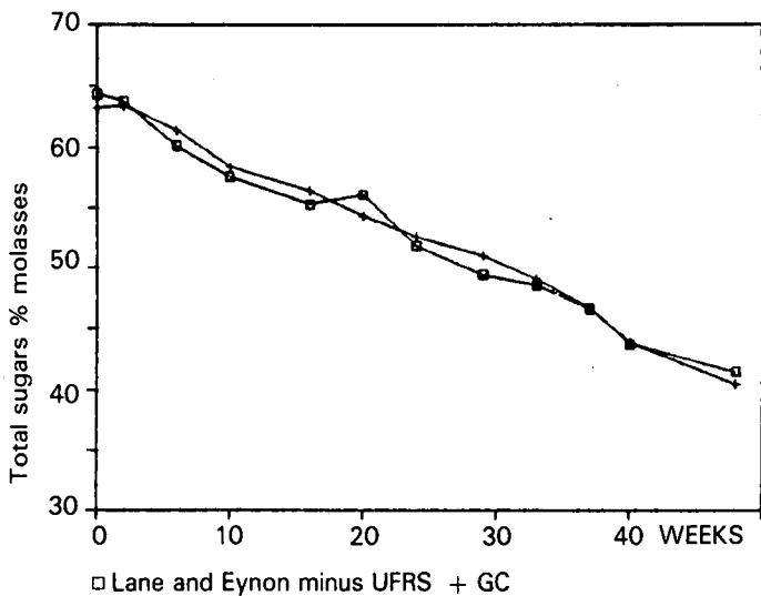
FIGURE 3 Total sugars by GC and by Lane & Eynon corrected for UFRS
