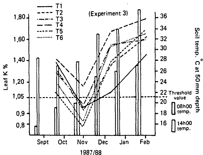
FIGURE 1 Changes in leaf K at various levels of applied K.
