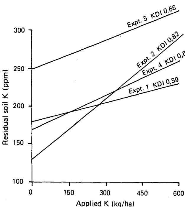
FIGURE 2 Relationship between applied K treatment and residual soil exchangeable K values.
