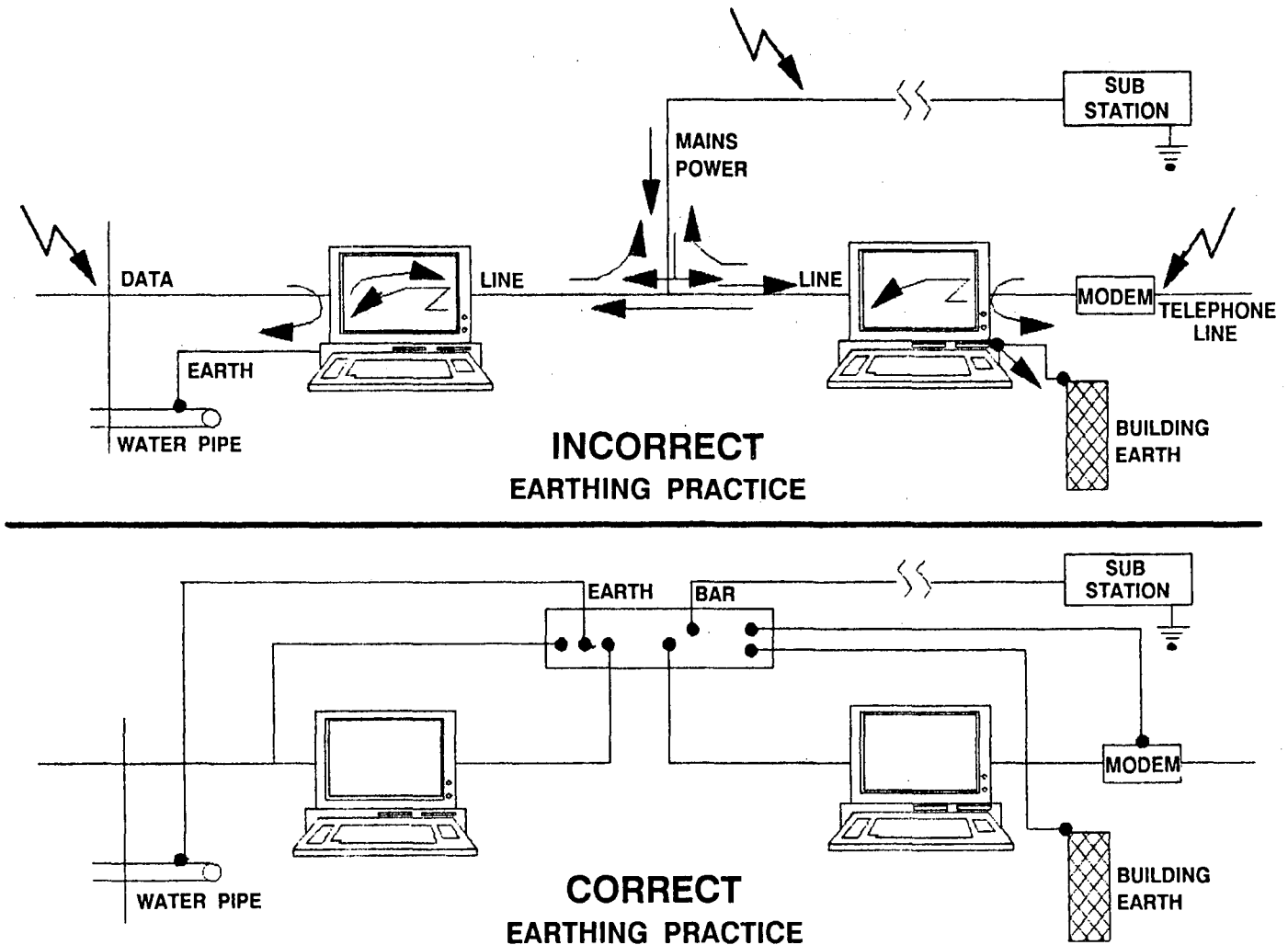
FIGURE 1 Examples of correct and incorrect earthing practices.
