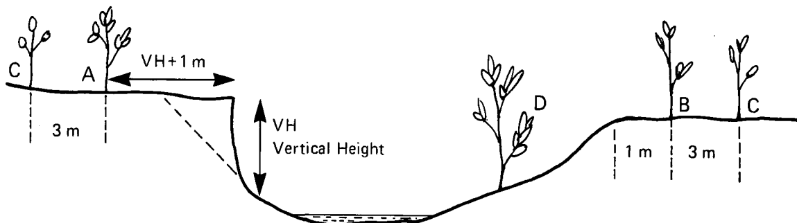
FIGURE 2 Cross-section of eroded bank of perennial stream.
