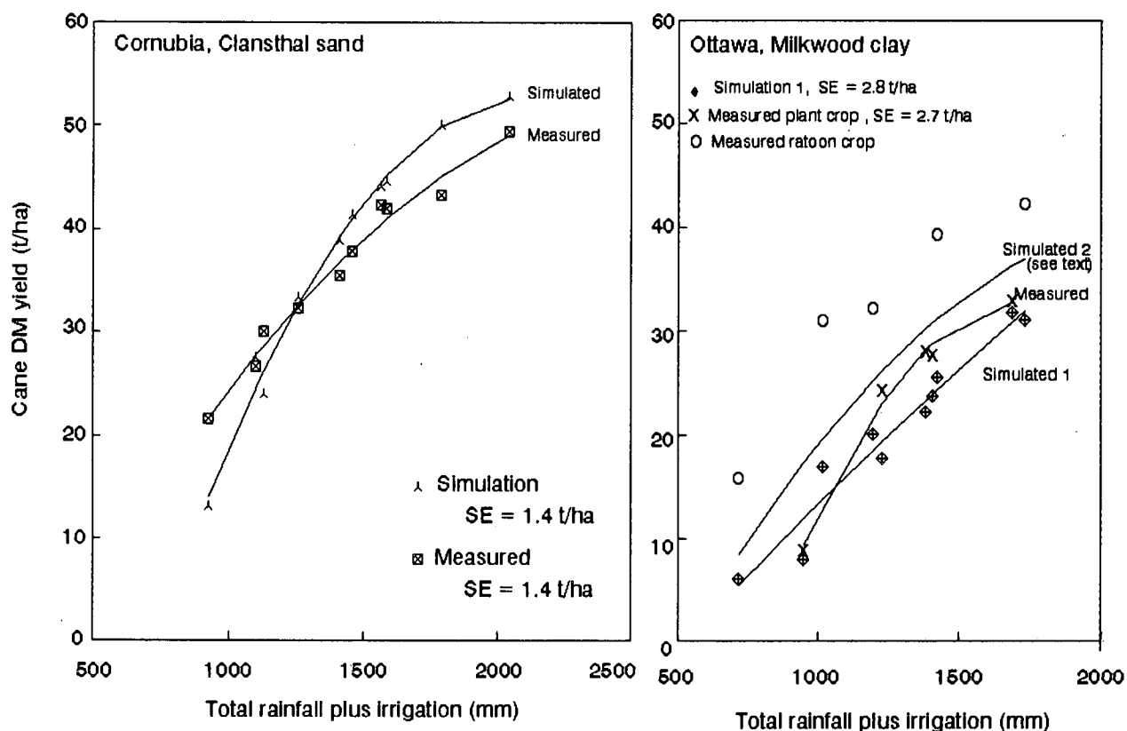
FIGURE 6 Simulated and measured yields in relation to rainfall plus different levels of net irrigation applied to two crops of NCo376 in two experiments near Mount Edgecombe from 1964 to 1967.
