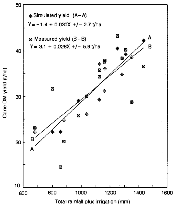
FIGURE 7 Simulated and measured yields in relation to rainfall plus different levels of net irrigation applied to five crops of NCo376 in an experiment at Pongola conducted from 1970 to 1976.
