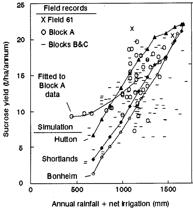
FIGURE 8 Simulated sucrose yield response to rain plus net irrigation for three soils on an estate in northern Natal and the association between recorded yield and net irrigation plus rainfall for fields with Hutton form soils.
