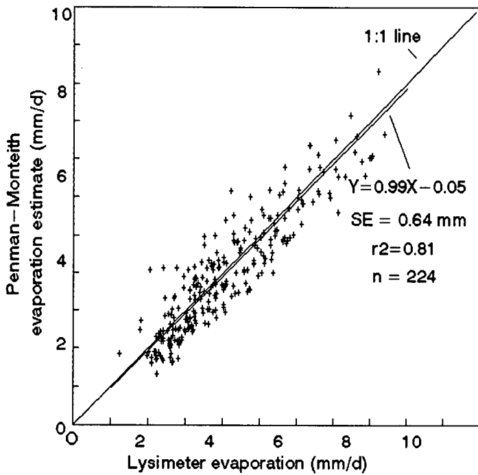
FIGURE 2 Estimated and measured daily evaporation of NCo376 growing in three lysimeters at Pongola, from the 50% canopy stage onwards. Co-ordinates are means of the three lysimeters and weighted (1:2:1) three-day running means.
