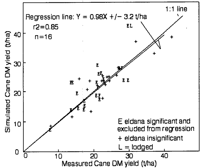
FIGURE 4 Simulated and measured yields of NCo376 in nine variety trials on a Shortlands form soil conducted at Mtunzini from 1978 to 1992.
