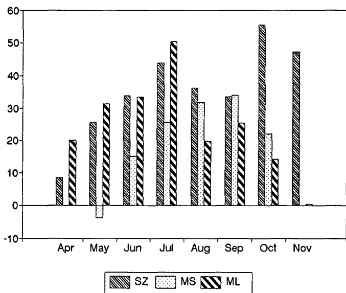
FIGURE 7 Percent difference in the non-sucrose throughput at SZ, MS and ML, 1991/92 and 1992/93 seasons.
