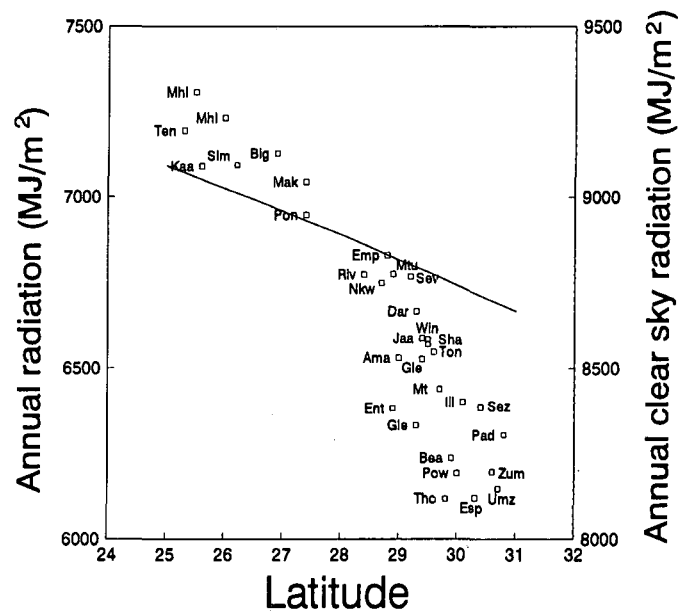
FIGURE 1 Mean annual solar radiation (□) and clear sky radiation (—) for weather stations at various latitudes in the SA sugar industry. Note that the range for the Y-axes differ but not the scale.
