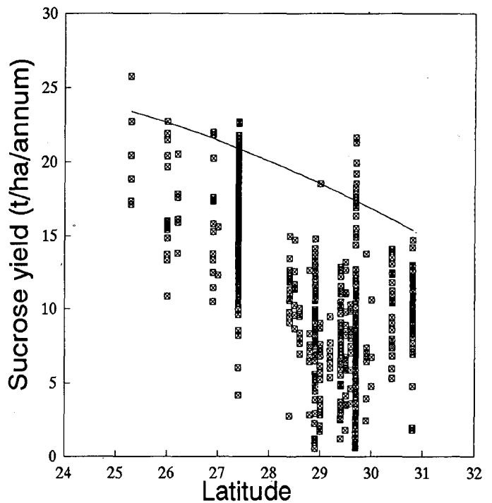
FIGURE 3 Annualised sucrose yields of NCo376 from all released variety trials conducted at different latitudes and radiation-limited sucrose yield potential obtained by simulation and from equation (1) in text for 100 m altitude.
