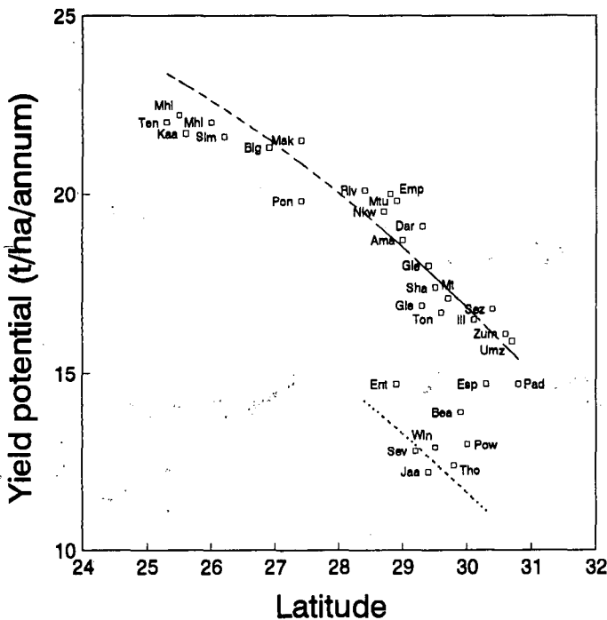
FIGURE 2 Mean annual sucrose yield (□) limited only by radiation and temperature, obtained by simulation for weather stations at various latitudes and curves fitted by least squares for altitudes of 100 m (---) and 1 000 m (.....).
