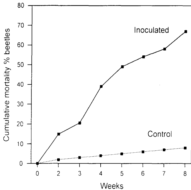
Figure 1. Effect of the fungus Metarhizium anisopliae on Heteronychus licas in bioassay trials.
