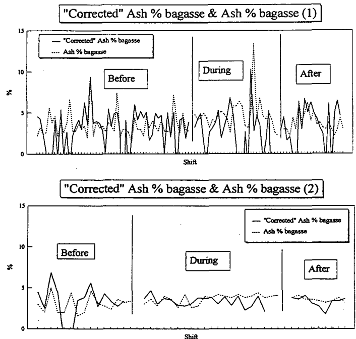
Figure 6. Ash in bagasse trends for Trials 1 and 2.
