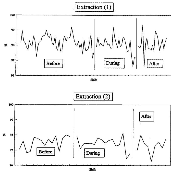
Figure 2. Extraction trends for Trials 1 and 2.
