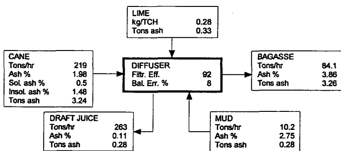
Figure 5. Ash mass balance for Trial 2.
