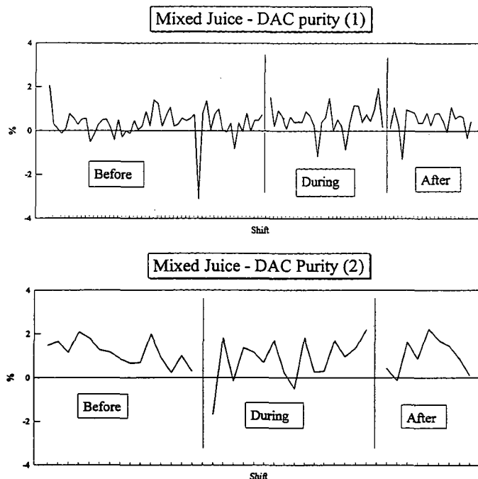
Figure 3. Draft juice minus DAC purity trends for Trials 1 and 2.
