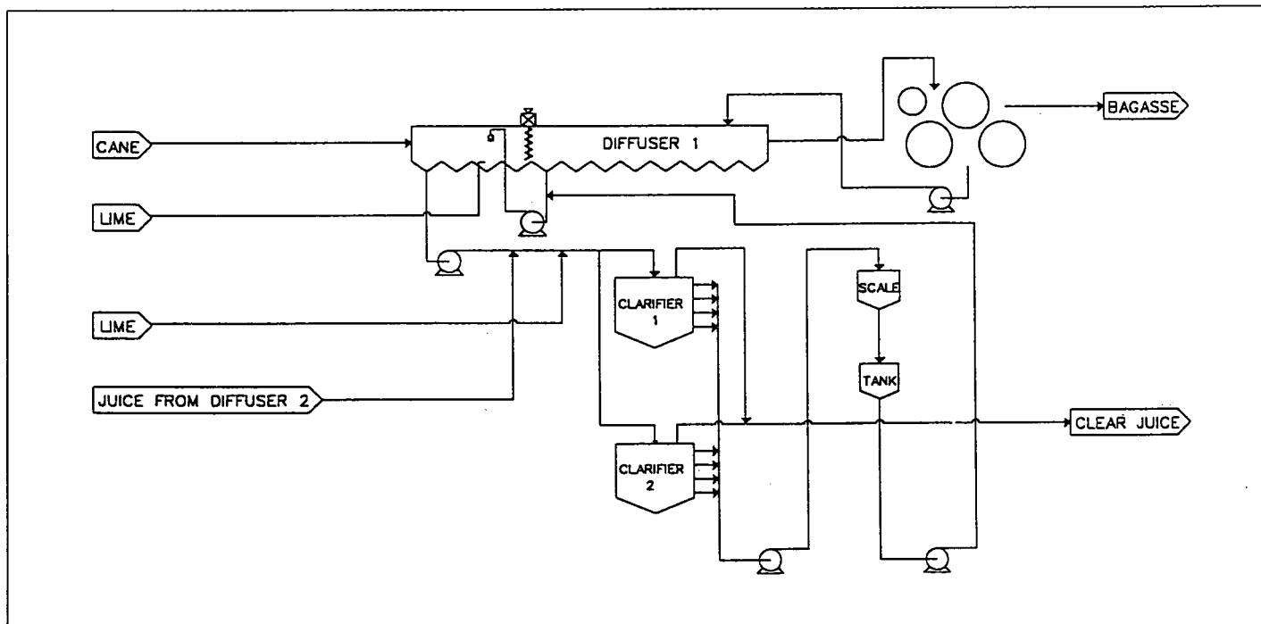
Figure 1: Process flow diagram of mud recycle.
