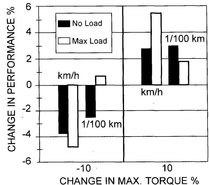
Figure 4. Sensitivity of speed and fuel consumption to 10% changes in the torque envelope (after Clark, 1996).
