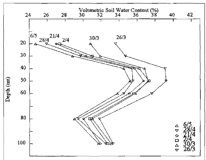
Figure 2c. Variations of 'Probe' estimated soil water, with respect to soil depth and time at Site Sable-N2B – checking the 'refill' point.
