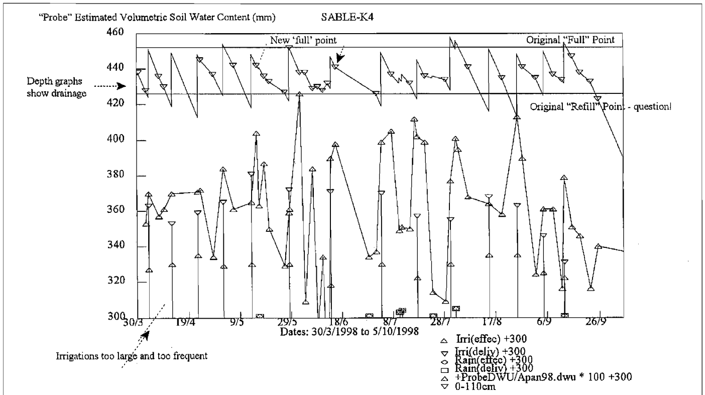
Figure 3a. Variations of 'Probe' estimated soil water, 'Probe' estimated daily water use (DWU) /A-pan, and effective delivered irrigations and rain.
