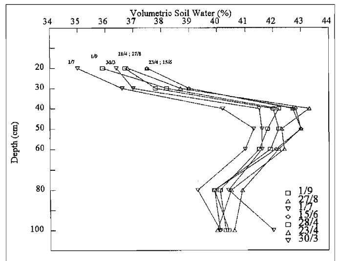
Figure 3c. Variations of 'Probe' estimated soil water, with respect to soil depth and time at Site Sable-K4.
