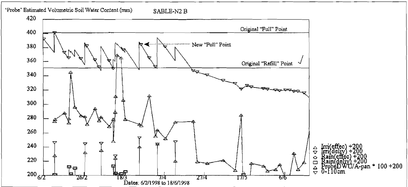
Figure 2a. Variations of 'Probe' estimated daily water use (DWU) /A-pan, and effective delivered irrigations and rain.
