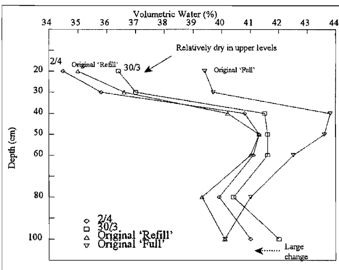
Figure 3b. Variations of 'Probe' estimated soil water, with respect to soil depth and time at Site Sable-K4.
