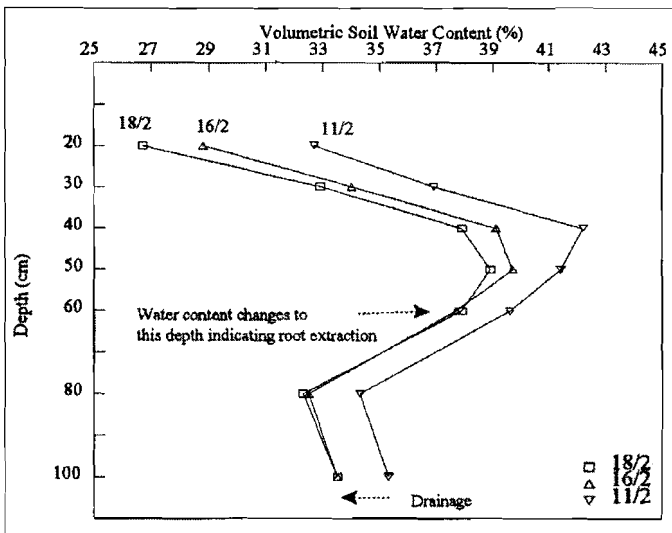
Figure 2b. Variations of 'Probe' estimated soil water, with respect to soil depth and time at Site Sable-N2B
