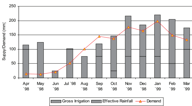
Figure 2. Typical overhead irrigation supply and demand curve at pump stations 13 and 14 at RSSC during the cropping season 98-99.
