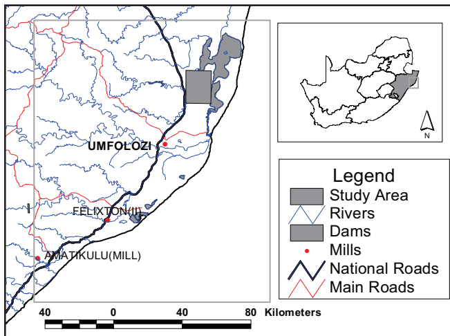
Figure 1. Map showing the location of the Umfolozi mill supply and study area.
