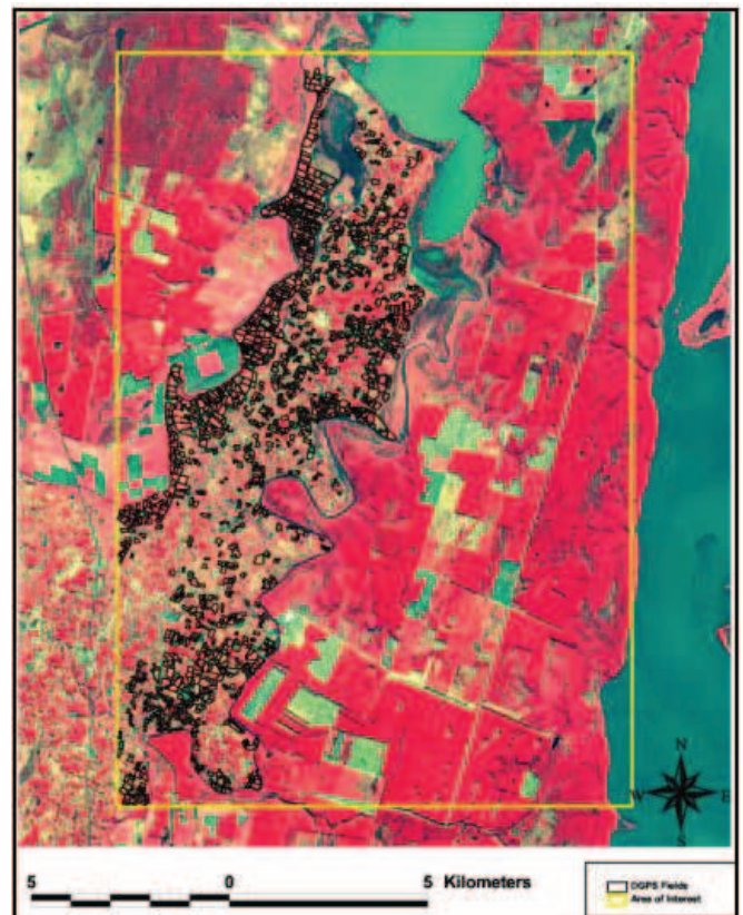
Figure 2. False colour composite satellite image (17 July 2000) showing the extent of the study area and field boundaries.
