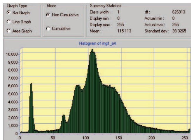
Figure 3. Histogram of the spectral reflectance values for the entire image for the fourth band (shortwave infrared) on 26 May 2000.
