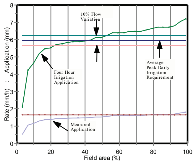
Figure 3. Graph to show in-field variation of water application for a four hour irrigation event with SSD irrigation.
