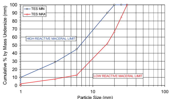
Figure 4. Preferred coal grading for high and low reactivity coal.
