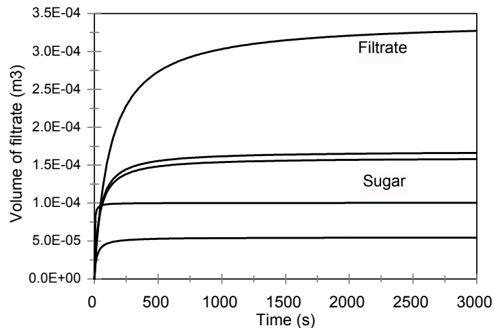
Figure 4. Filtration rates for original and filtered solutions
