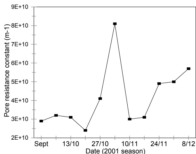
Figure 7. PRC values for the SAST samples
