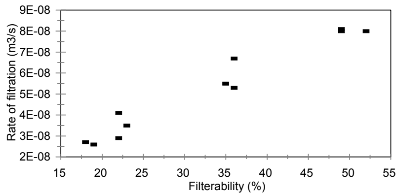
Figure 5. The relationship between DV/DT and percent filterability, SAST samples
