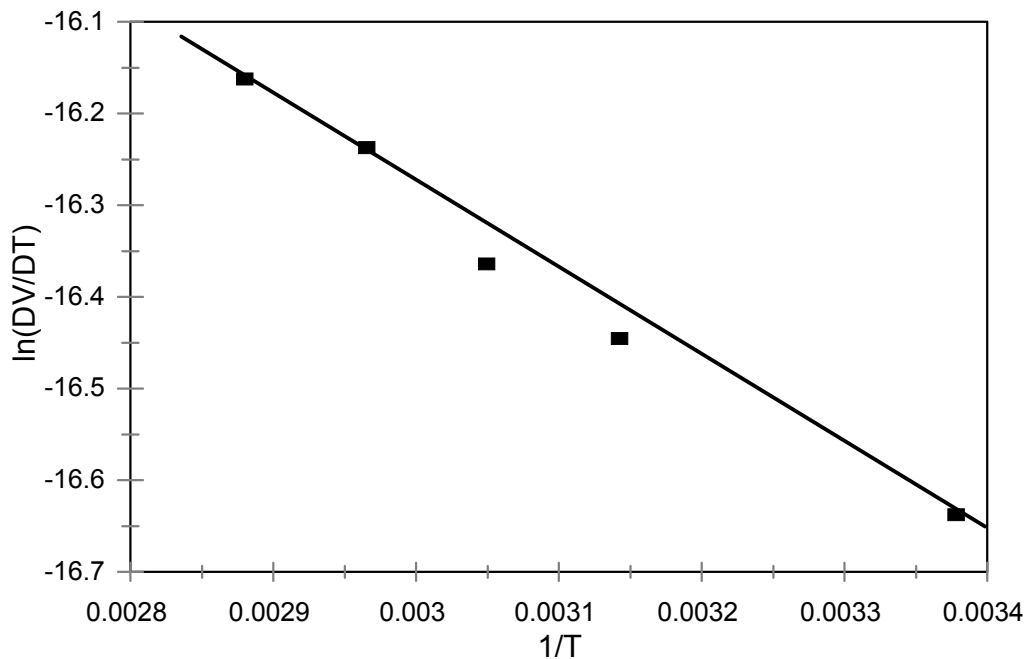
Figure 1. Arrhenius plot for the effect of temperature on the rate of filtration
