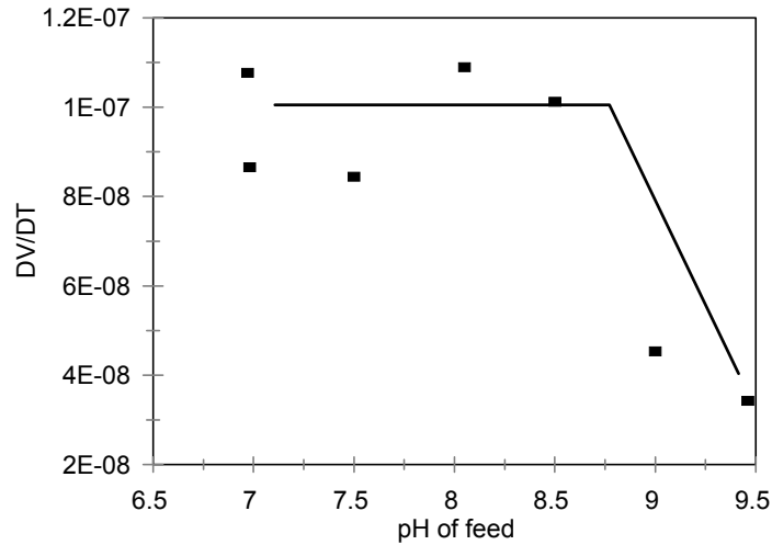
Figure 3. Effect of pH on the rate of filtration
