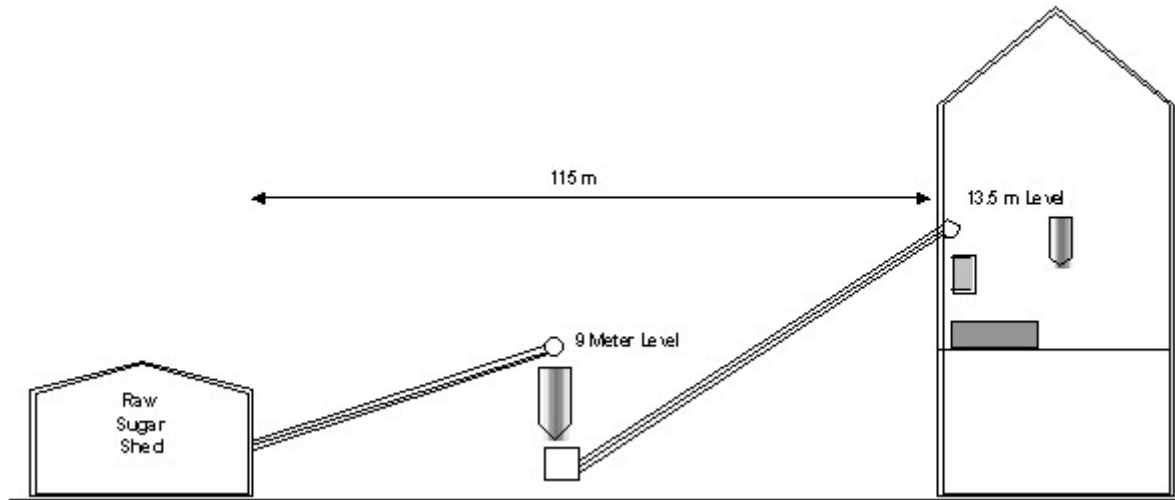
Figure 5. Arrangement of conveyors during Periods I and II.
