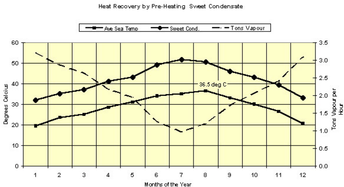
Figure 10. Heat recovery obtained by using 25 kPa (a) waste vapour.
