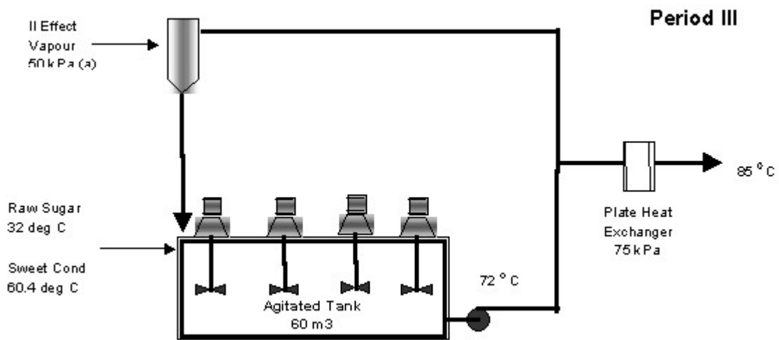
Figure 7. Configuration with new four-chambered agitated tank.
