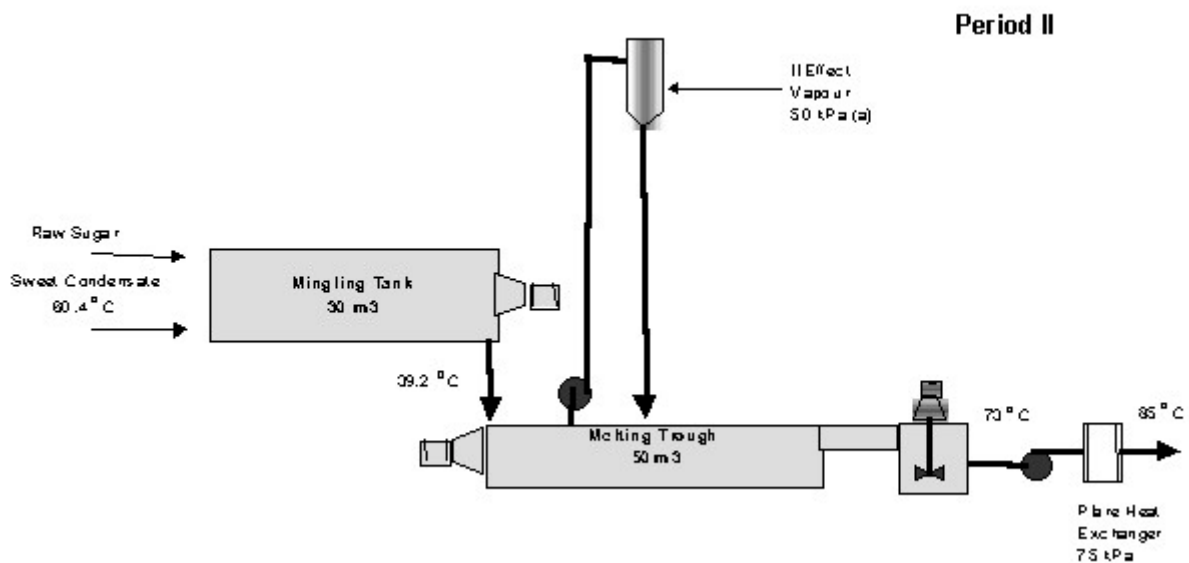
Figure 6. Configuration utilising external contact heater exchanger.
