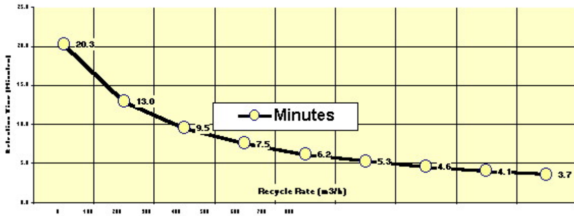
Figure 2. Sharp drop in retention time as the recycle rate increases.
