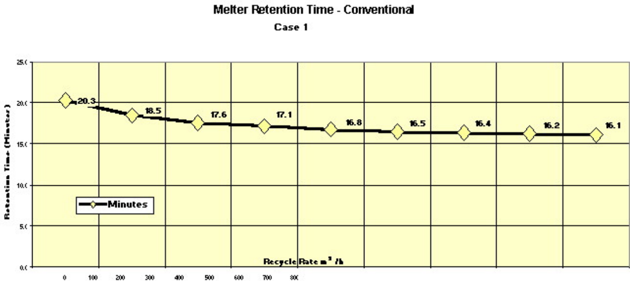
Figure 1. Relatively high retention time despite increasing the recycle rate.
