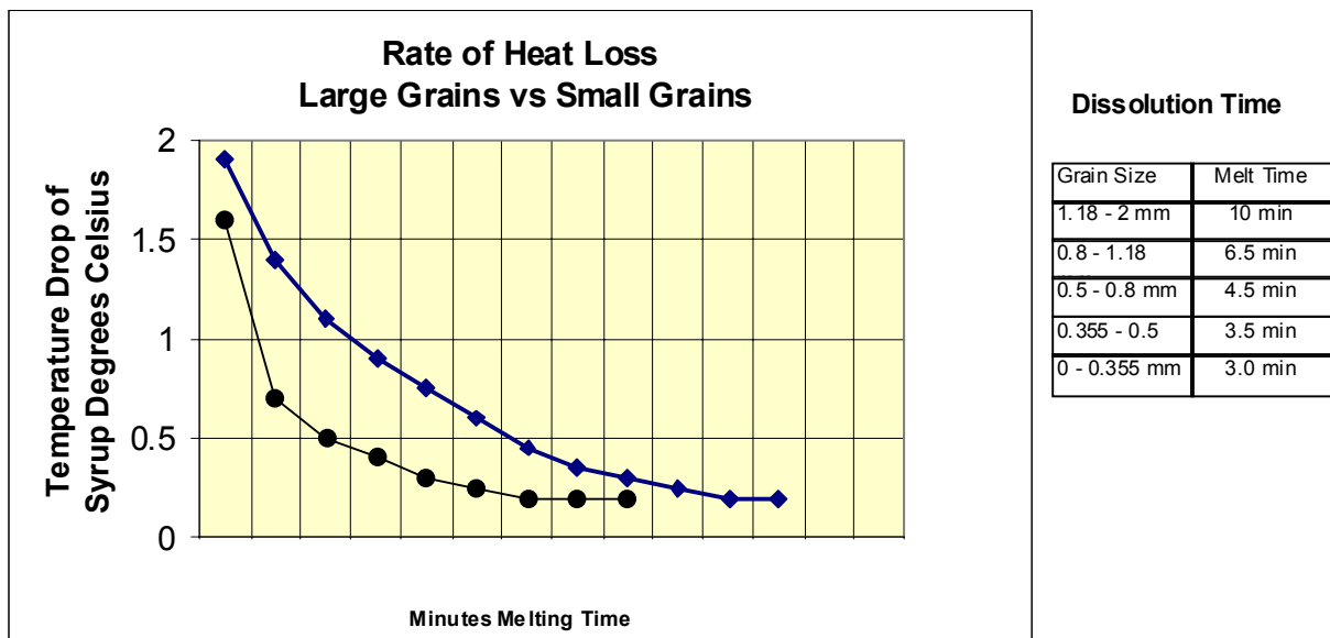
Figure 13. Heat loss during dissolution test.
