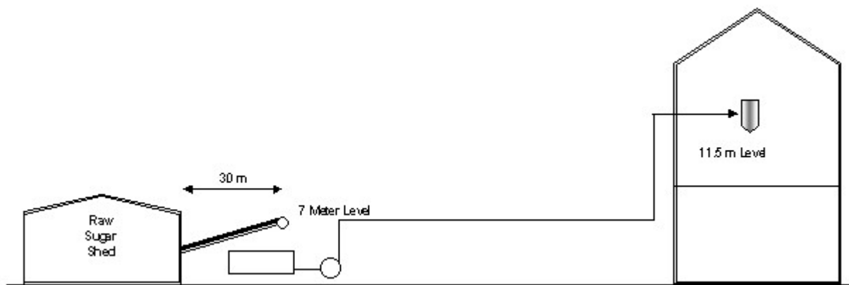
Figure 8. Arrangement of conveyors in Periods III and IV.
