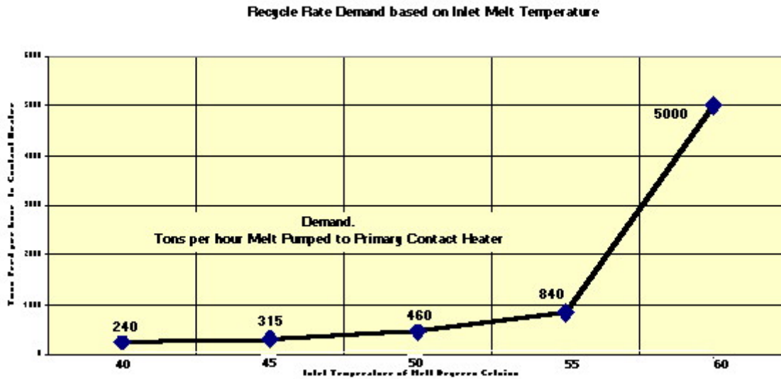
Figure 3. The influence of melter inlet temperature on recycle demand.
