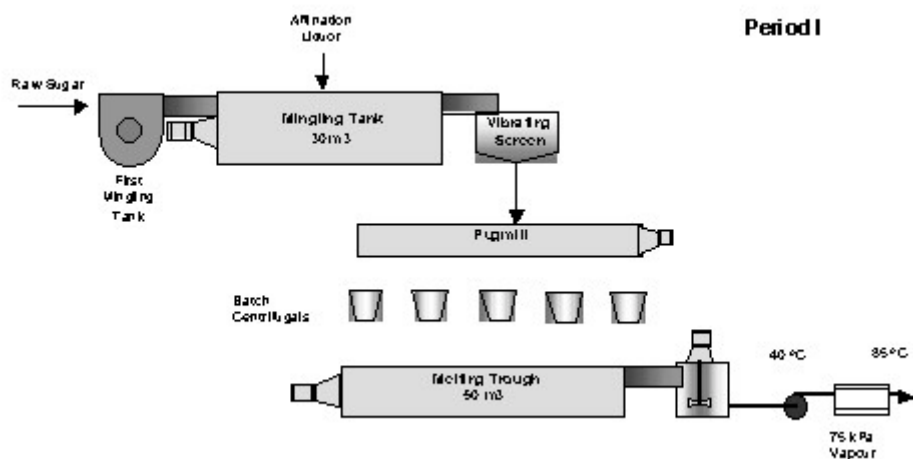
Figure 4. Original melter scheme incorporating the affination process.
