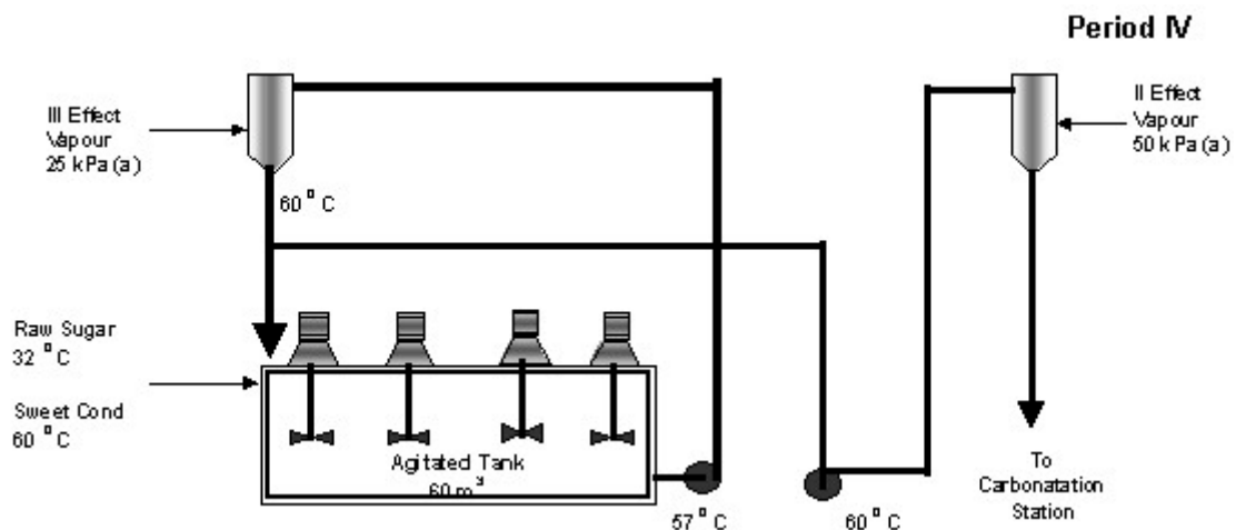
Figure 9. Configuration with two contact heaters in series.
