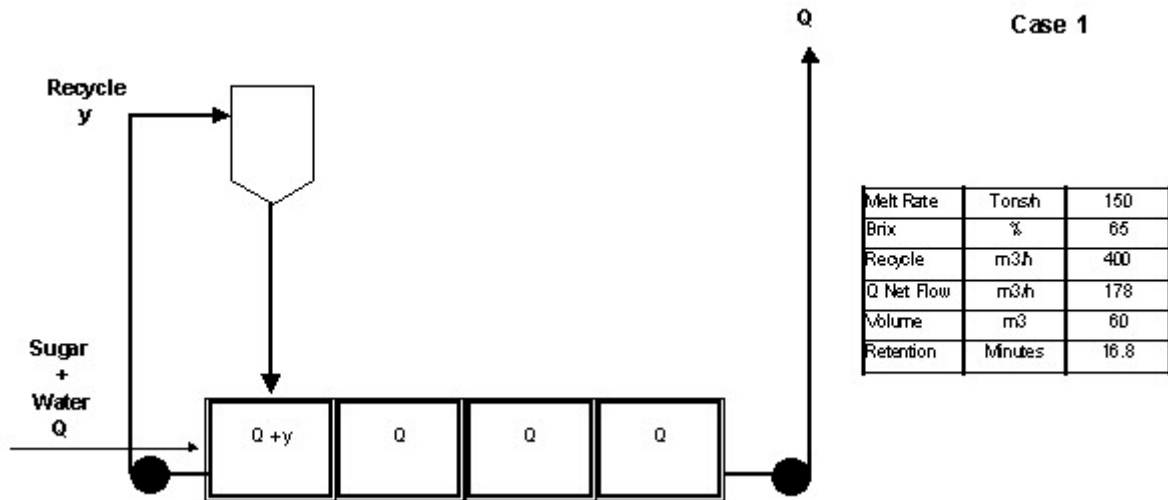
Figure 11. Case 1 recycle configuration.
