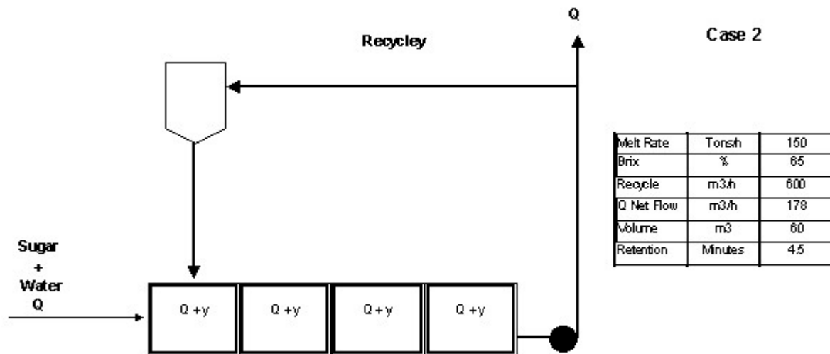
Figure 12. Case 2 recycle configuration.
