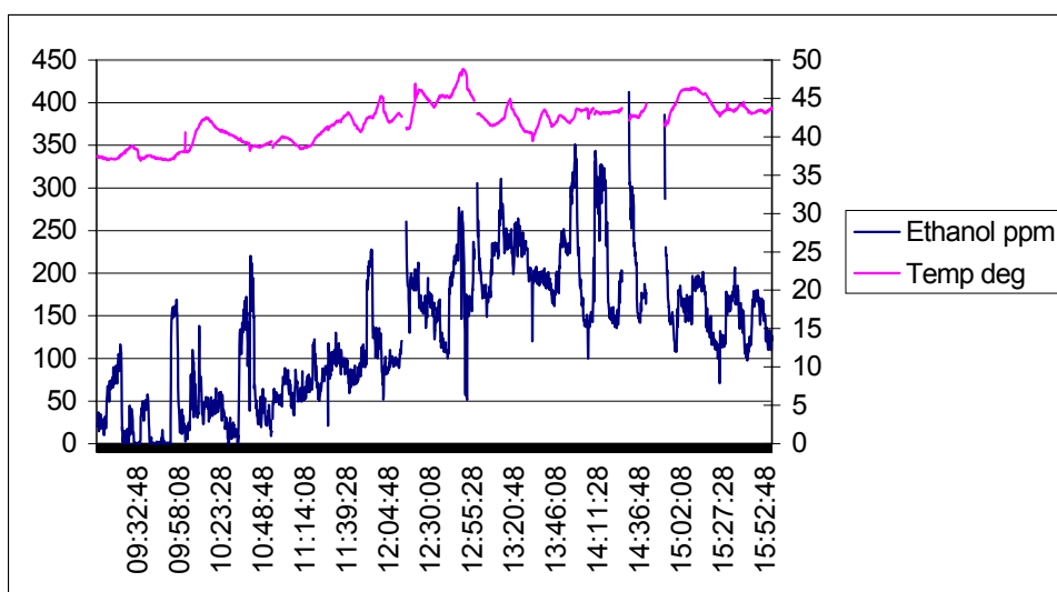
Figure 3. Temperature and detector reading against time.
