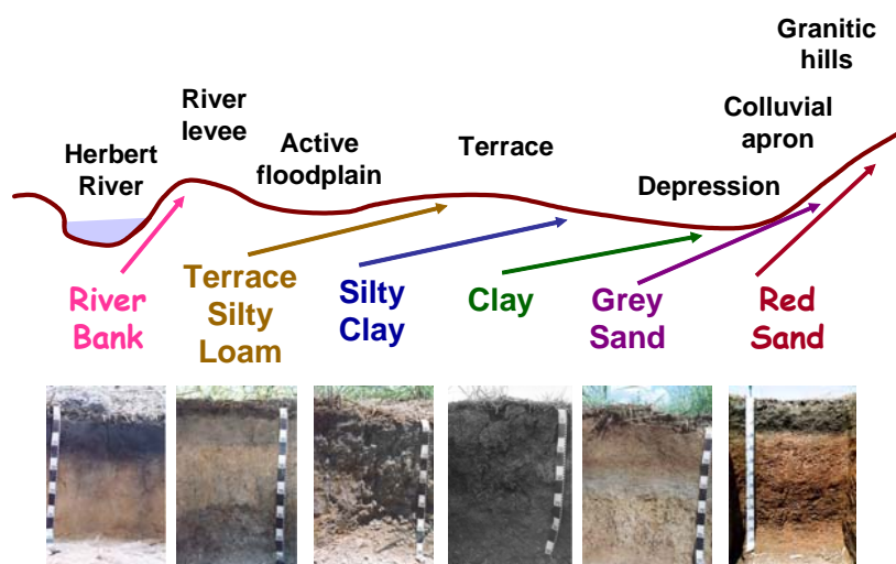
Figure 1. Example of a sequence of soils found in a typical landscape close to the Lower Herbert River (Wood et al. , 2003b).
