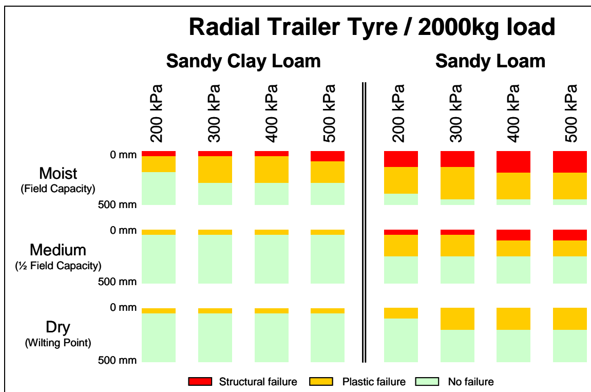
Figure 2. Soil damage profiles for permutations of different SOCOMO input variables (soil texture, moisture content and tyre inflation pressure).
