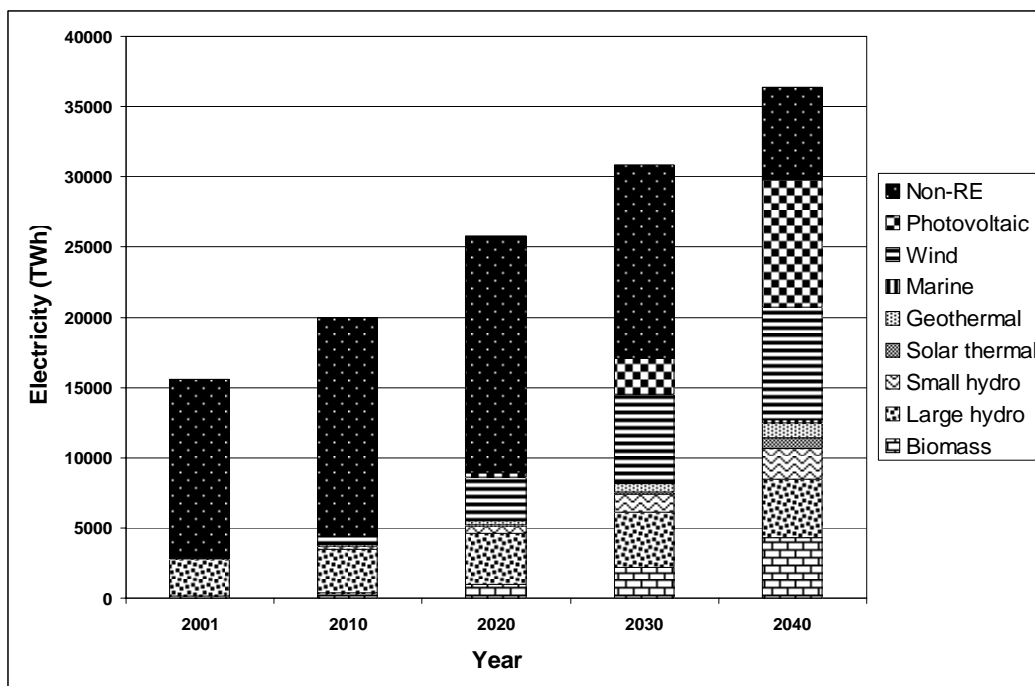
Figure 1. A 'high road' scenario for the contribution of renewable energy to world electricity generation (European Council on Renewable Energies, 2006 2 ).
