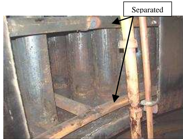
Figure 2. Pipes for light and heavy incondensable gases separated.
