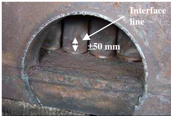
Figure 6. Condensate level of \pm 50 mm at condensate outlet.
