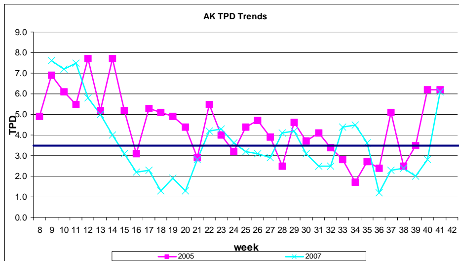
Figure 9. Comparison of target purity difference (TPD) trends at Amatikulu mill in 2005 and 2007.
