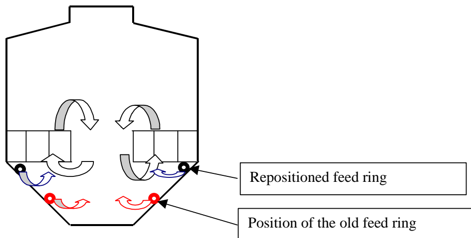
Figure 3. Representation of circulation pattern inside Pan 5 at Amatikulu mill, showing repositioned feed ring.
