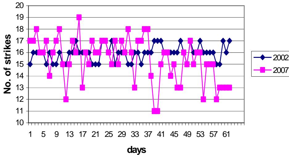
Figure 8. Comparison of maximum strikes achieved per day in August and September 2002 and for the same period in 2007 at Amatikulu mill.
