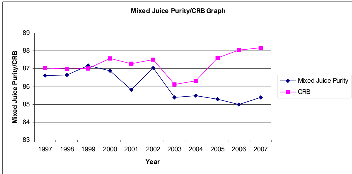
Figure 10. Mixed juice purity and corrected reduced boiling house recovery (CRB) at Amatikulu from 1997 to 2007.
