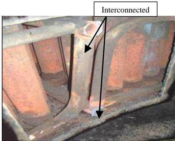
Figure 1. Pipes for light and heavy incondensable gases interconnected inside calandria.
