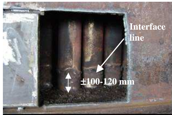
Figure 7. Condensate level of \pm 100-120 mm and soft scale on calandria tube plate.
