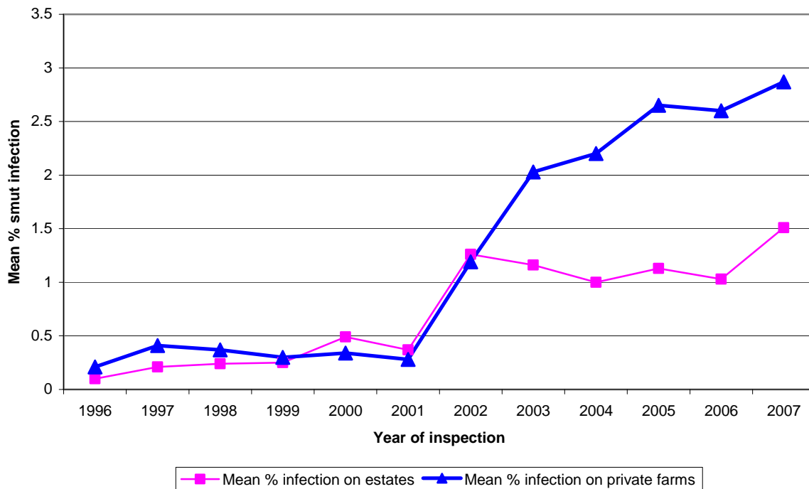
Figure 3. Weighted mean % smut infection in variety NCo376, showing the increase in the incidence of smut on privately owned farms compared to the incidence on estates following the Land Reform Programme introduced in 2001 in Zimbabwe.
