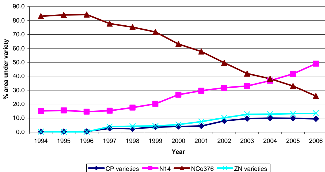
Figure 2. Percentage area in the Zimbabwe sugar industry grown to a single variety or group of varieties from 1994 to 2006. CP varieties were CP72-1312 and CP72-2086 bred at Canal Point, USA; ZN varieties were nine releases crossed in Natal, RSA, and selected in Zimbabwe.
