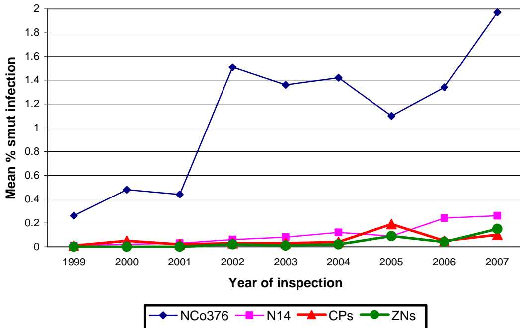
Figure 4. Mean % smut infection in the commercial varieties grown in Zimbabwe from 1999 to 2007.
