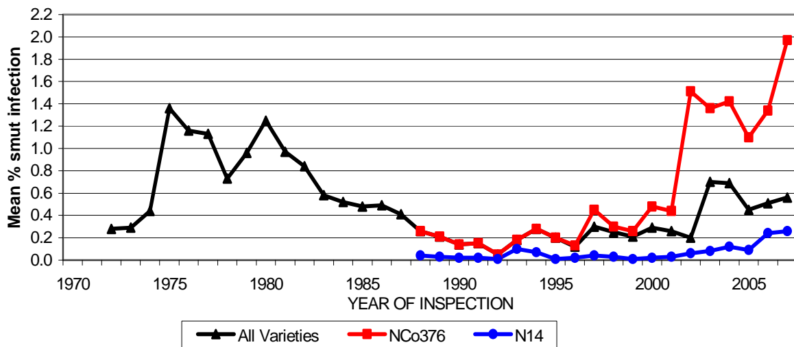
Figure 1. Mean annual % smut infection recorded in the Zimbabwe sugar industry from 1972 to 2007. 'All varieties' consisted of NCo376 and NCo310 up to 1979; mainly NCo376 up to 1985; NCo376 and N14 up to 1995; NCo376, N14, ZN1L, ZN2E and CP72-1312 up to 1999; and the 14 varieties released after 2000.
