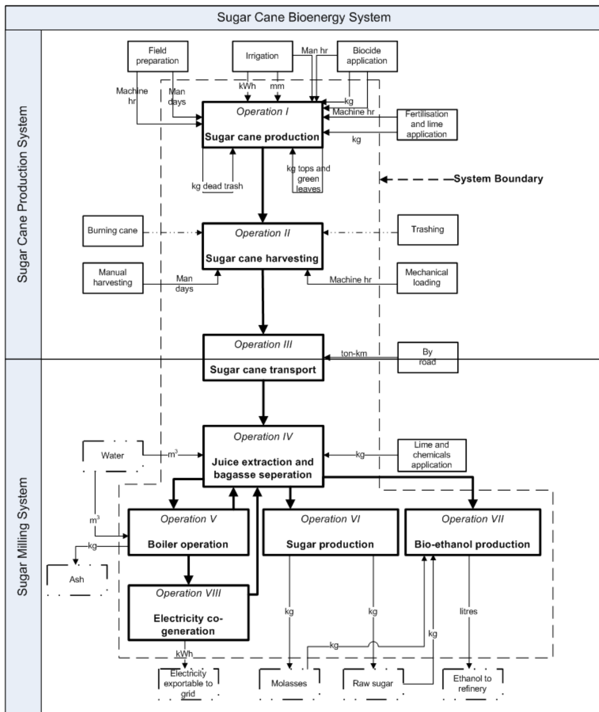
Figure 1. The sugarcane bioenergy system. Source: Adapted from Mohee and Beeharry (1999).
