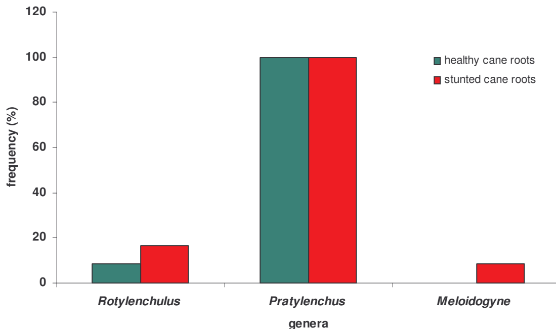
Figure 4. Percentage frequency of occurrence of nematode genera recovered from roots of healthy growing and stunted sugarcane.
