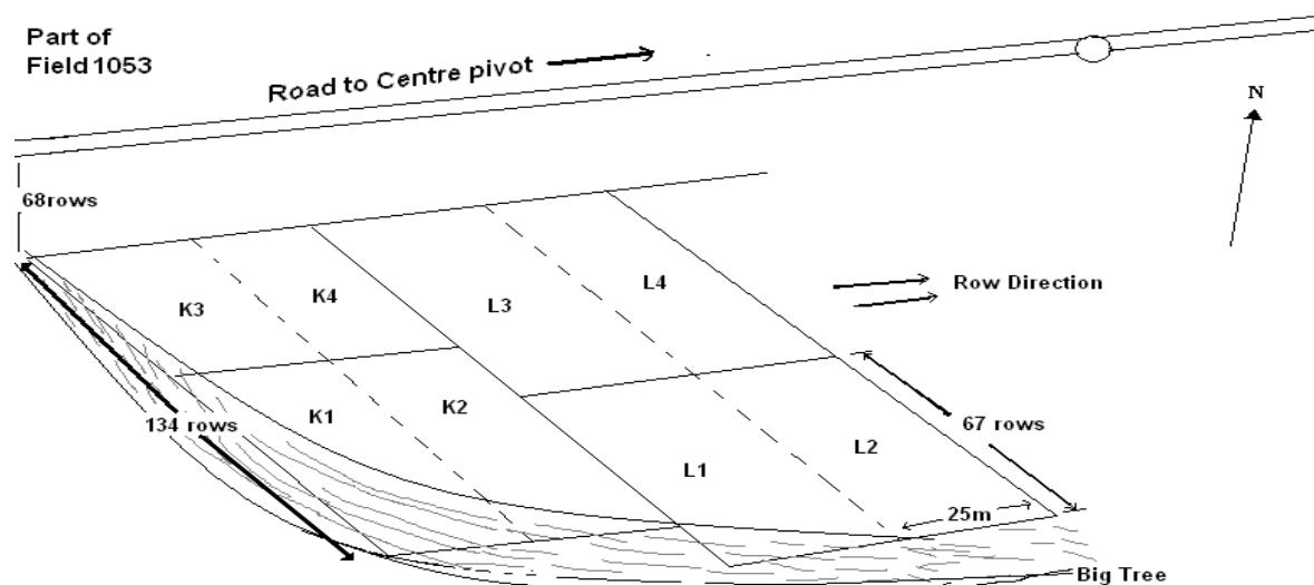
Figure 1b. Part of field 1053 at Section 10, Hippo Valley Estates, showing one-hectare blocks K and L, which were further subdivided into ¼ hectare plots (1-4). Areas with stunted cane are shaded.
