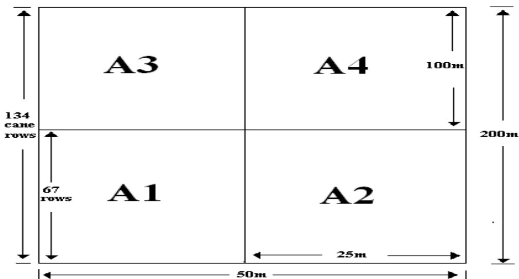
Figure 1c. Relative sizes of ¼ hectare plots (quadrants) in a one-hectare block. The letter (A) is the block label; the number (1-4) is the quadrant number. Each quadrant had 67 cane rows, spaced at 1.5 m (equivalent to 100 m) and was 25 m long.
