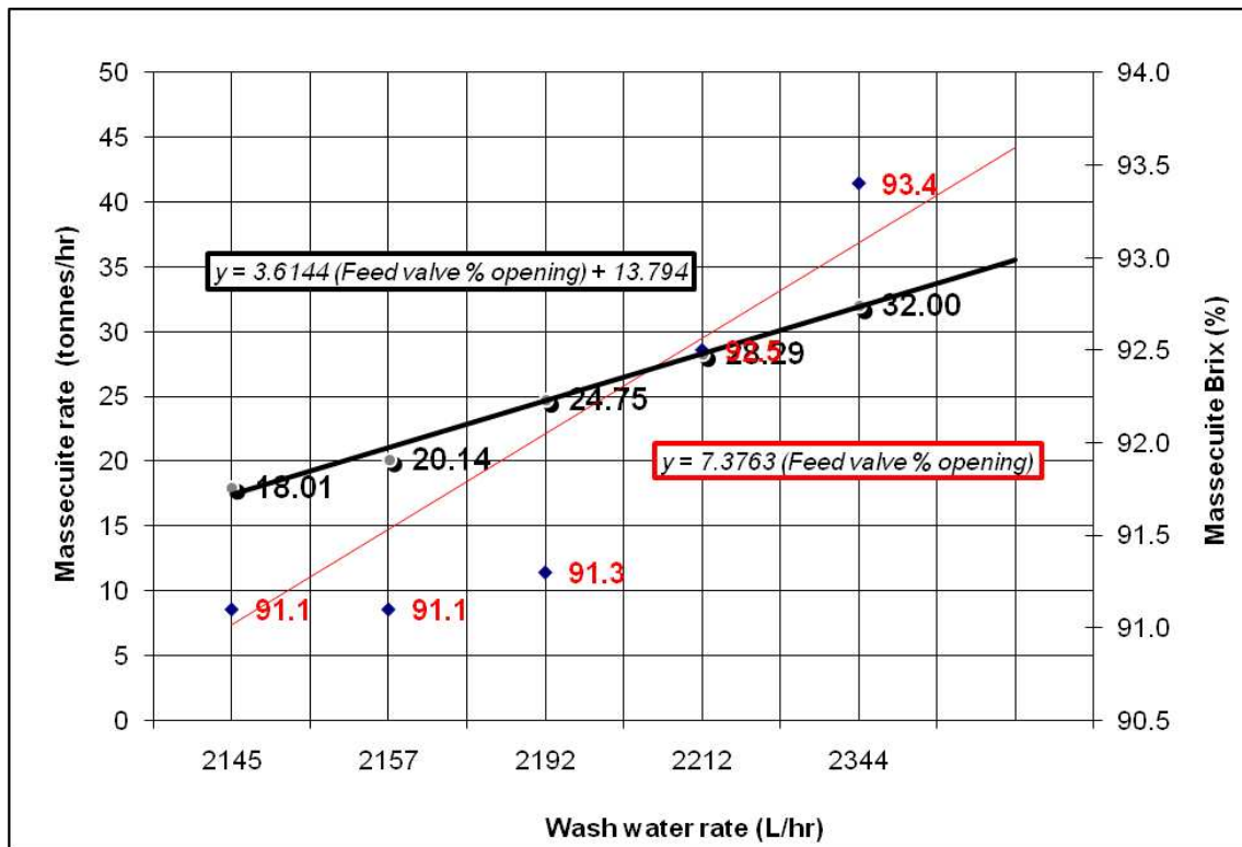
Figure 2. Relationship between massecuite throughput and massecuite feed valve (% open).
