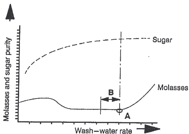
Figure 4. Relationship purity to wash water application.
