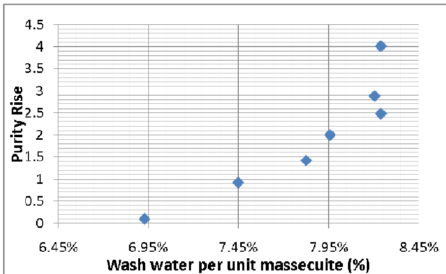
Figure 6. Purity rise as a function of wash % massecuite.
