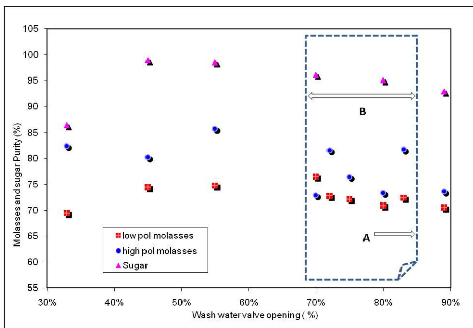
Figure 5. Relationship between sugar purity and molasses purity at varying wash water rates.
