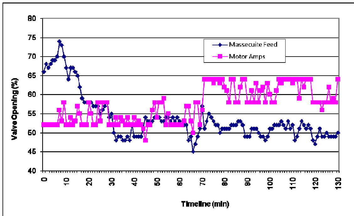
Figure 10. Masecuite feed rate as a function of power consumption (motor Amperage).
