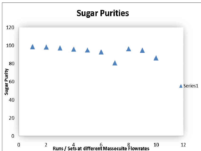
Figure 9. Sugar purities at different massecuite rates.
