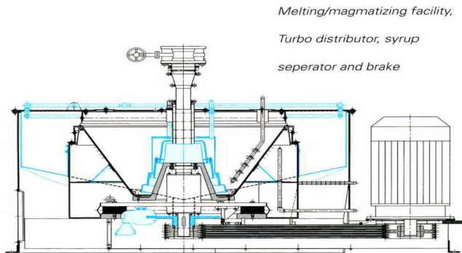
Figure 1. Schematic drawing of BMA k2300r continuous centrifugal.
