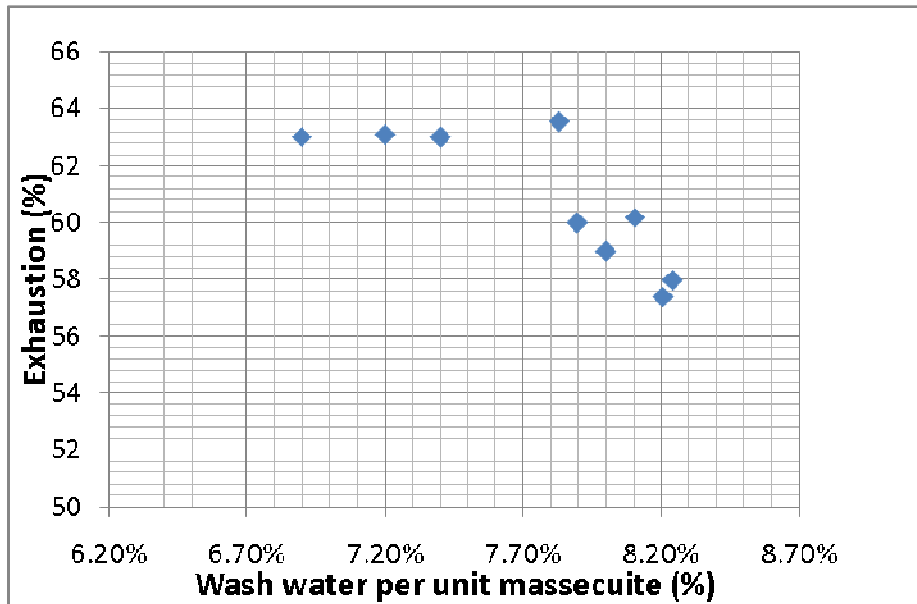
Figure 7. A-exhaustion as a function of wash % massecuite.
