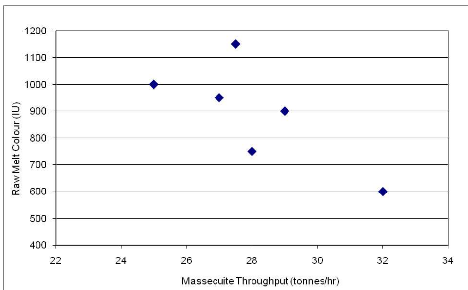
Figure 8. Melt colours at different massecuite throughput.
